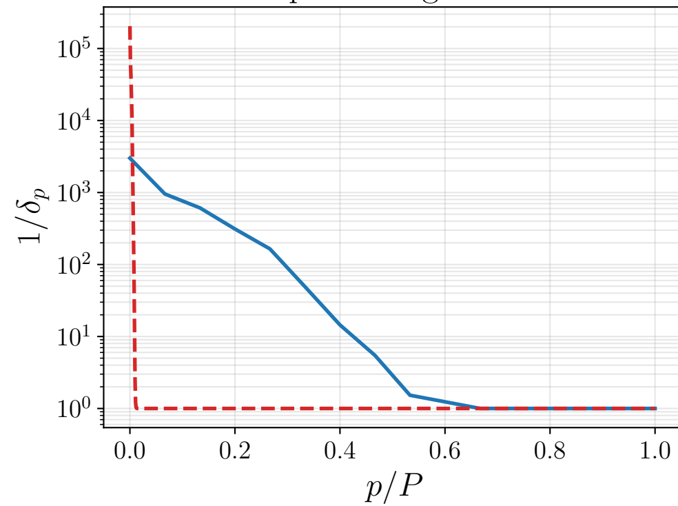
Reciprocal Eigenvalues
