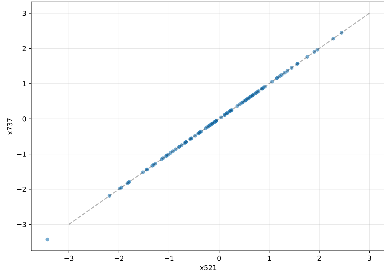
Input Space (Correlated)
