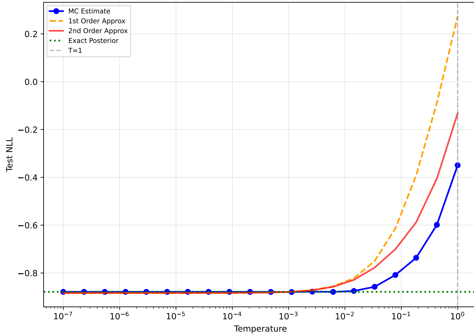
NLL Approximations ( \sigma_x = 1.0 )
