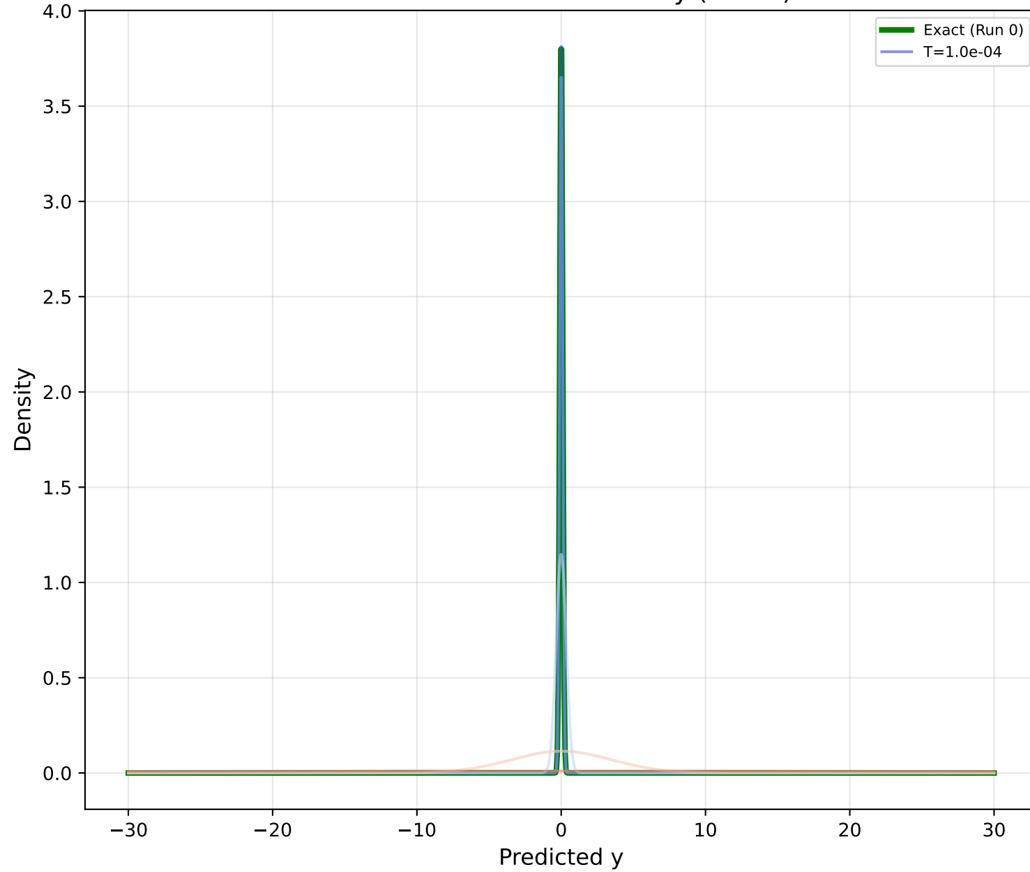
Posterior Predictive Density (Run 0)
