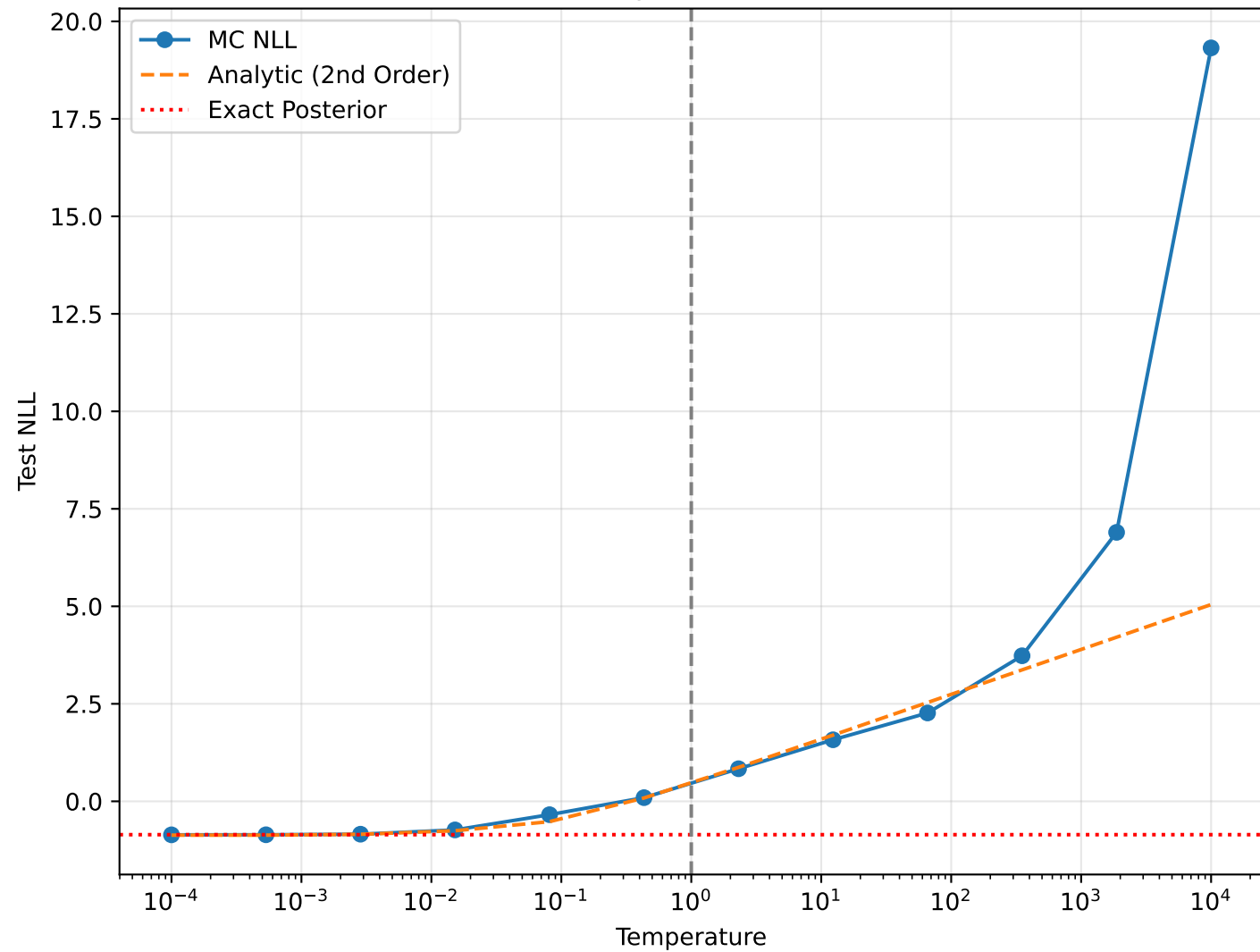
NLL vs Temperature (D=1024)
