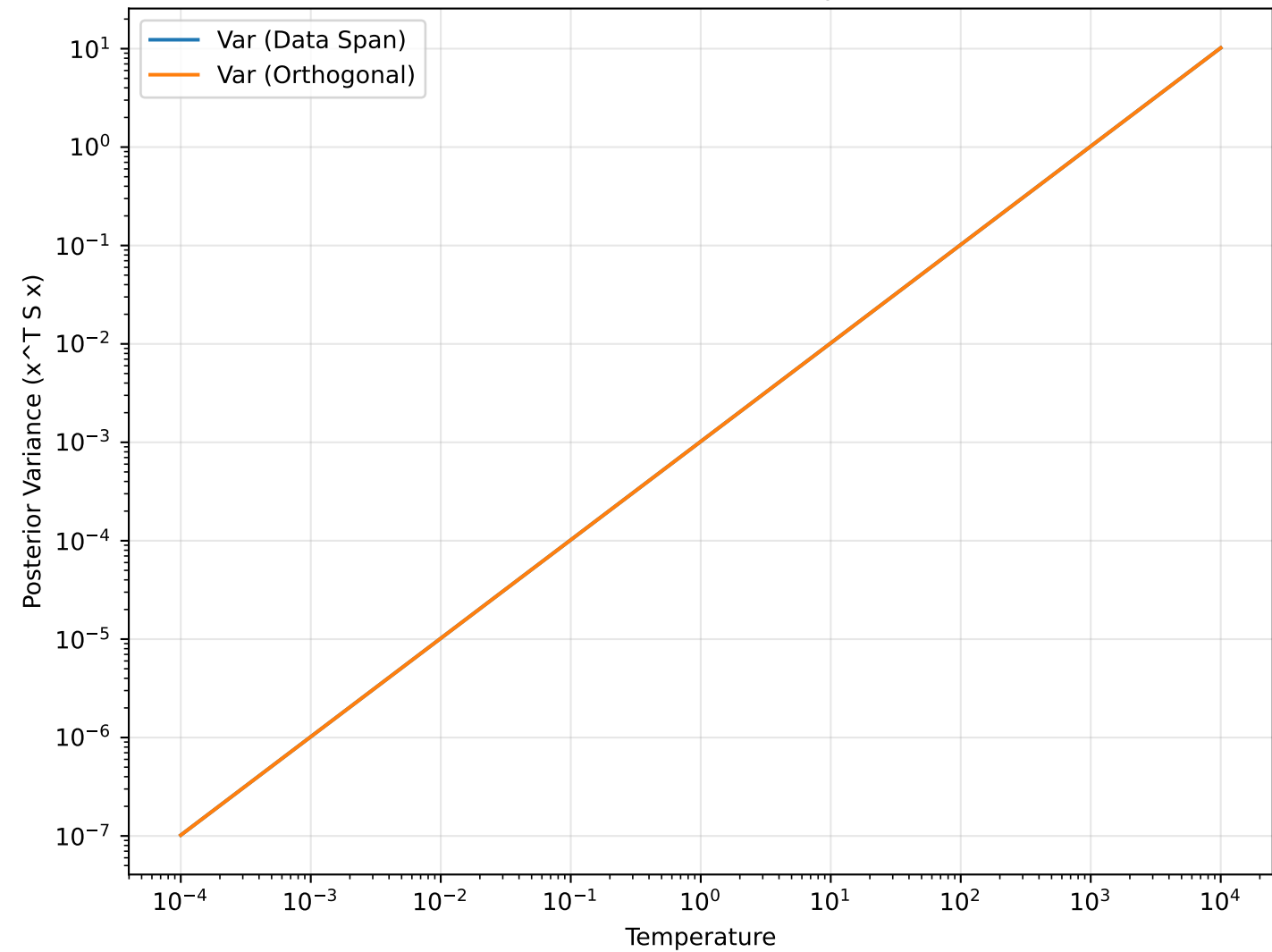
Directional Variance Components
