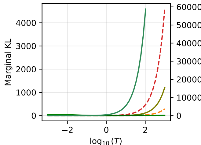
power
