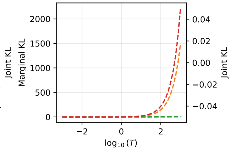
protein
