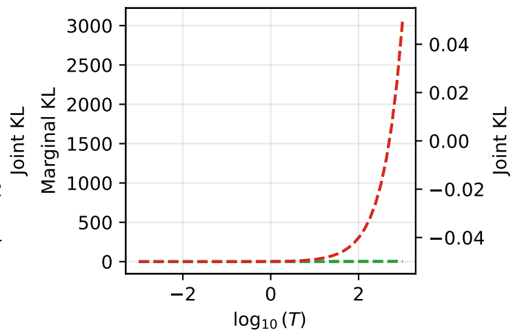
naval
