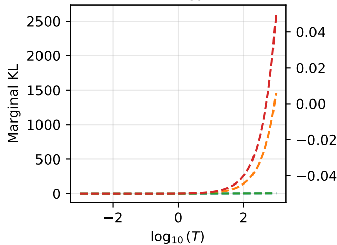
wine
