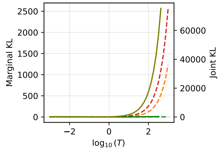
yacht
