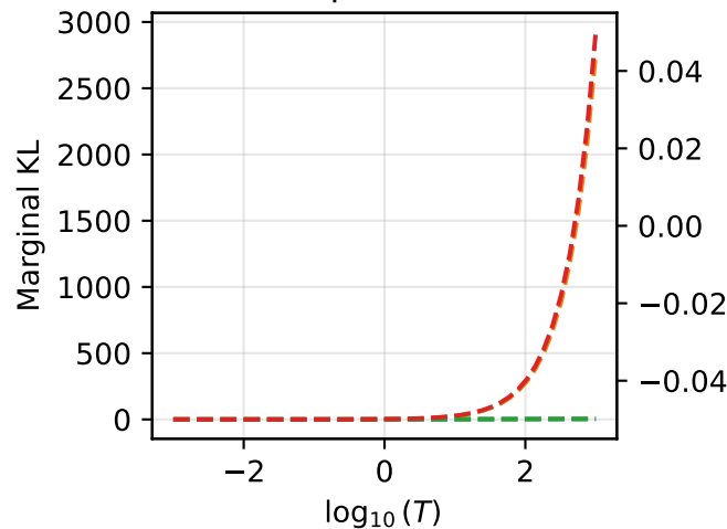
power
