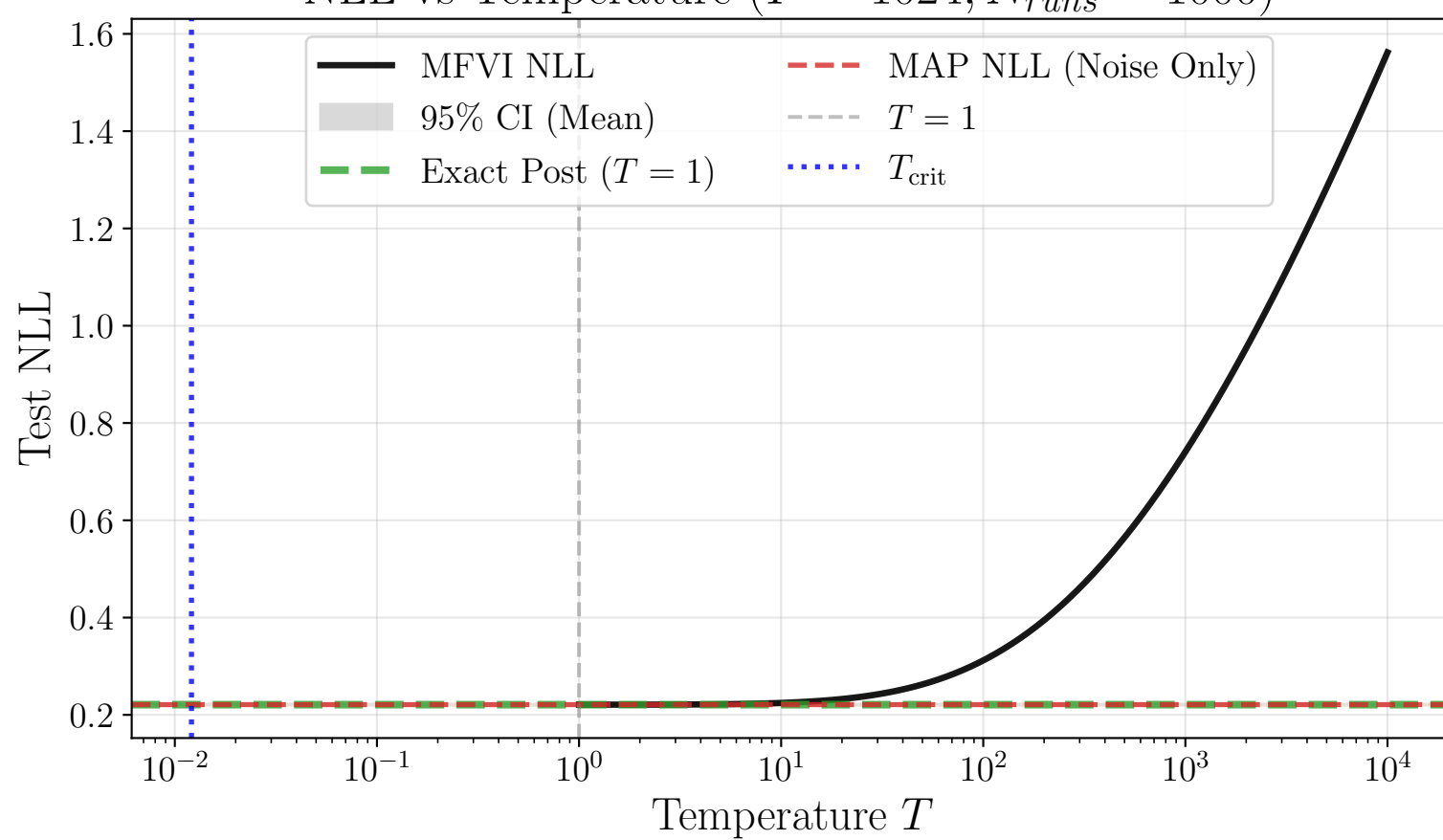
NLL vs Temperature ( P = 1024, N_{runs} = 1000 )
