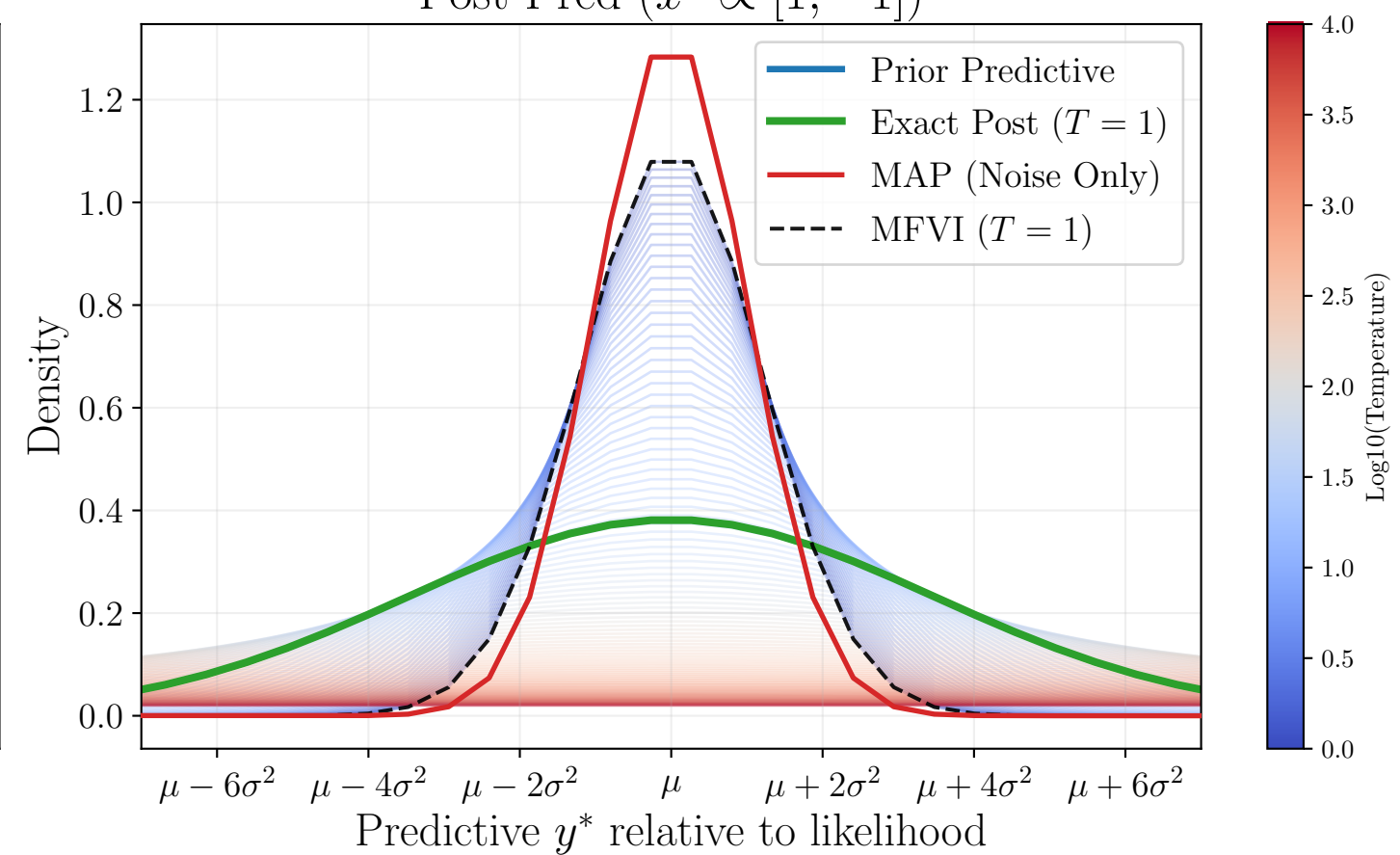
Post Pred ( x^* \propto [1, \dots, 1, -1, \dots, -1] )
