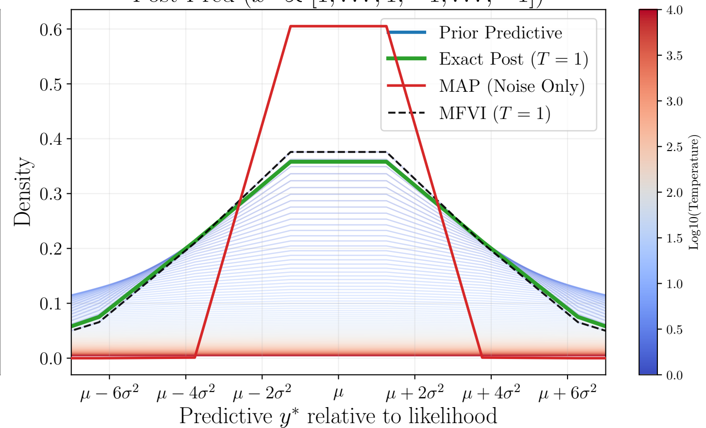
Post Pred ( x^* \propto [1, \dots, 1, -1, \dots, -1] )
