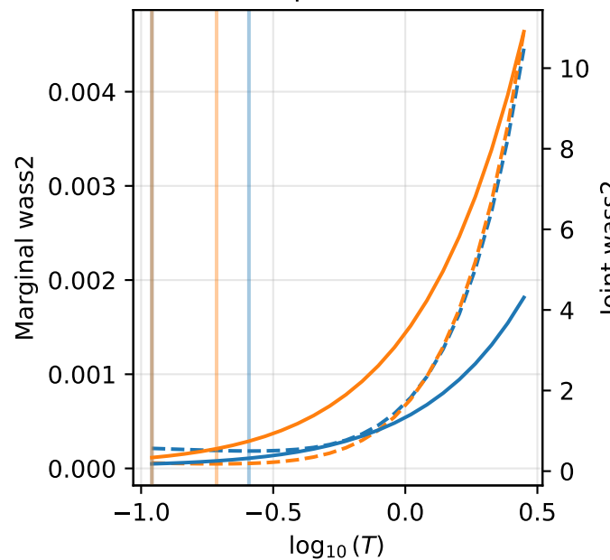
power
