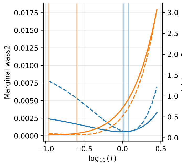
power
