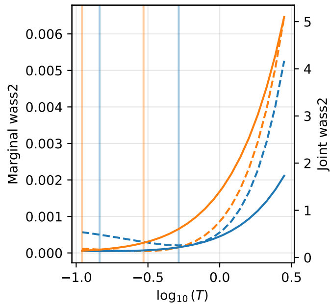
yacht
