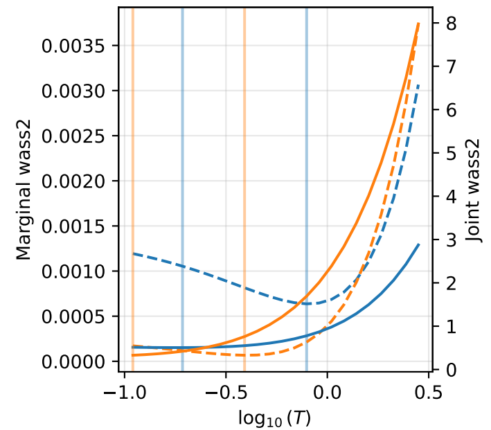
protein
