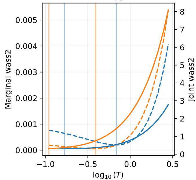
wine
