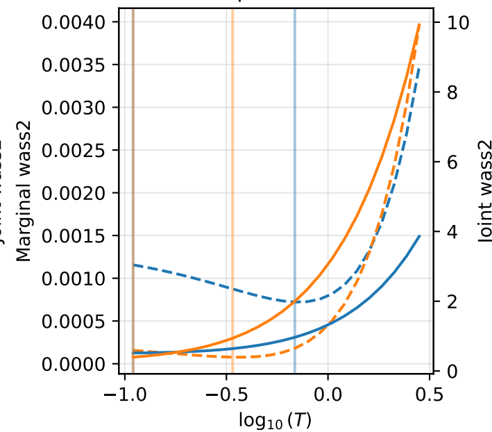
naval
