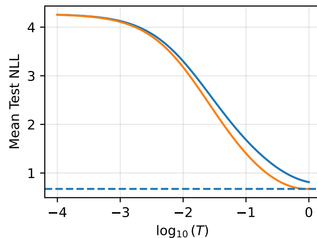
power
