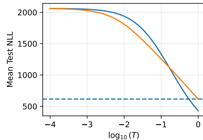
protein
