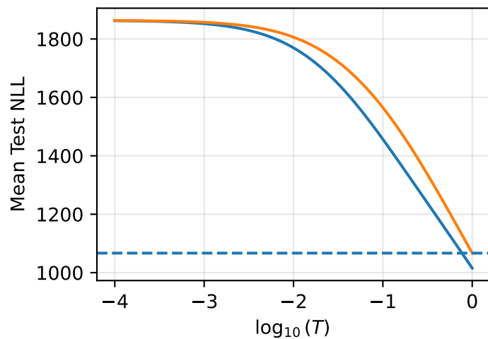
yacht
