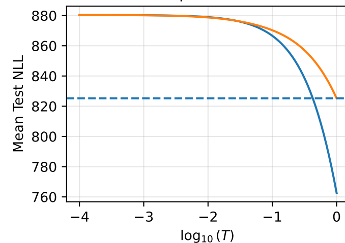
naval
