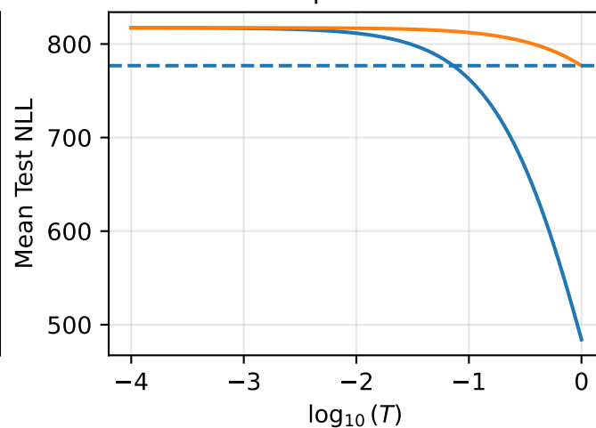
power
