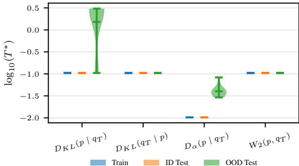
Joint divergences
