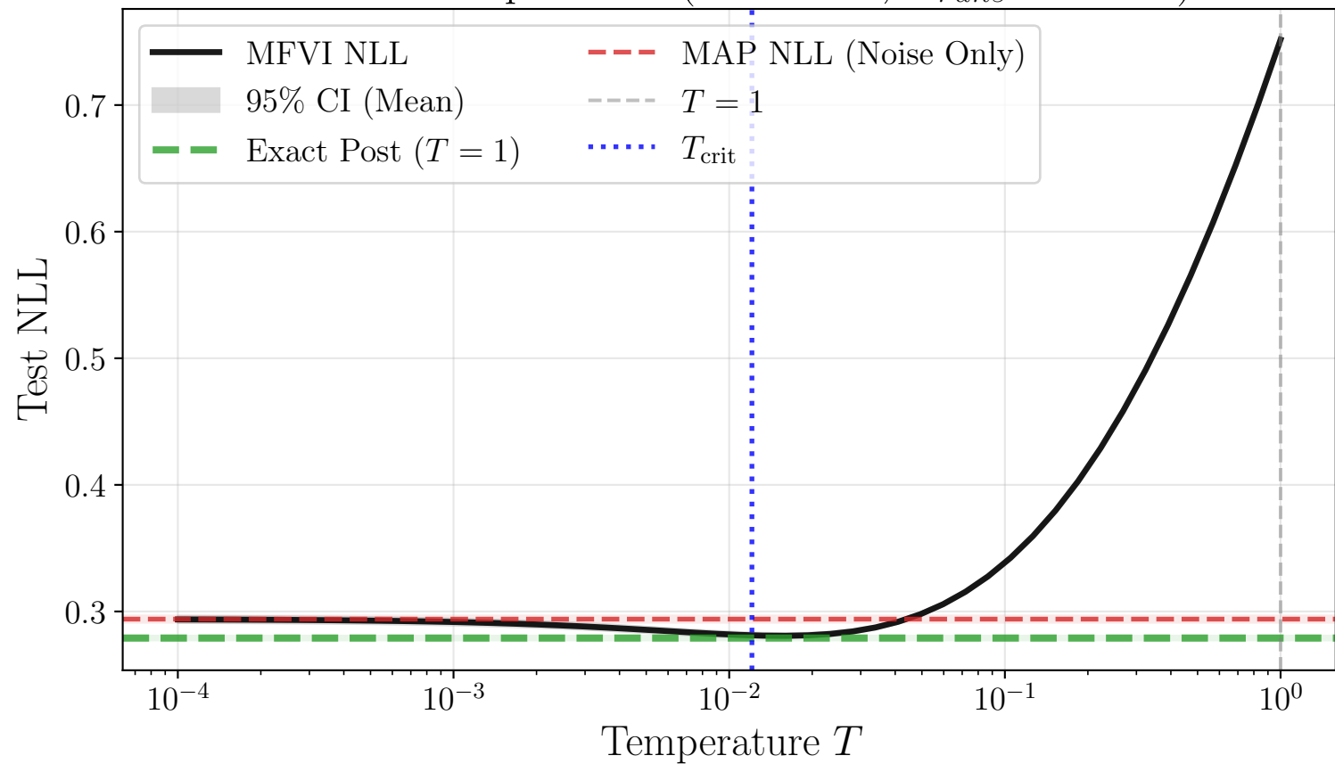
NLL vs Temperature ( P = 1024, N_{runs} = 10000 )
