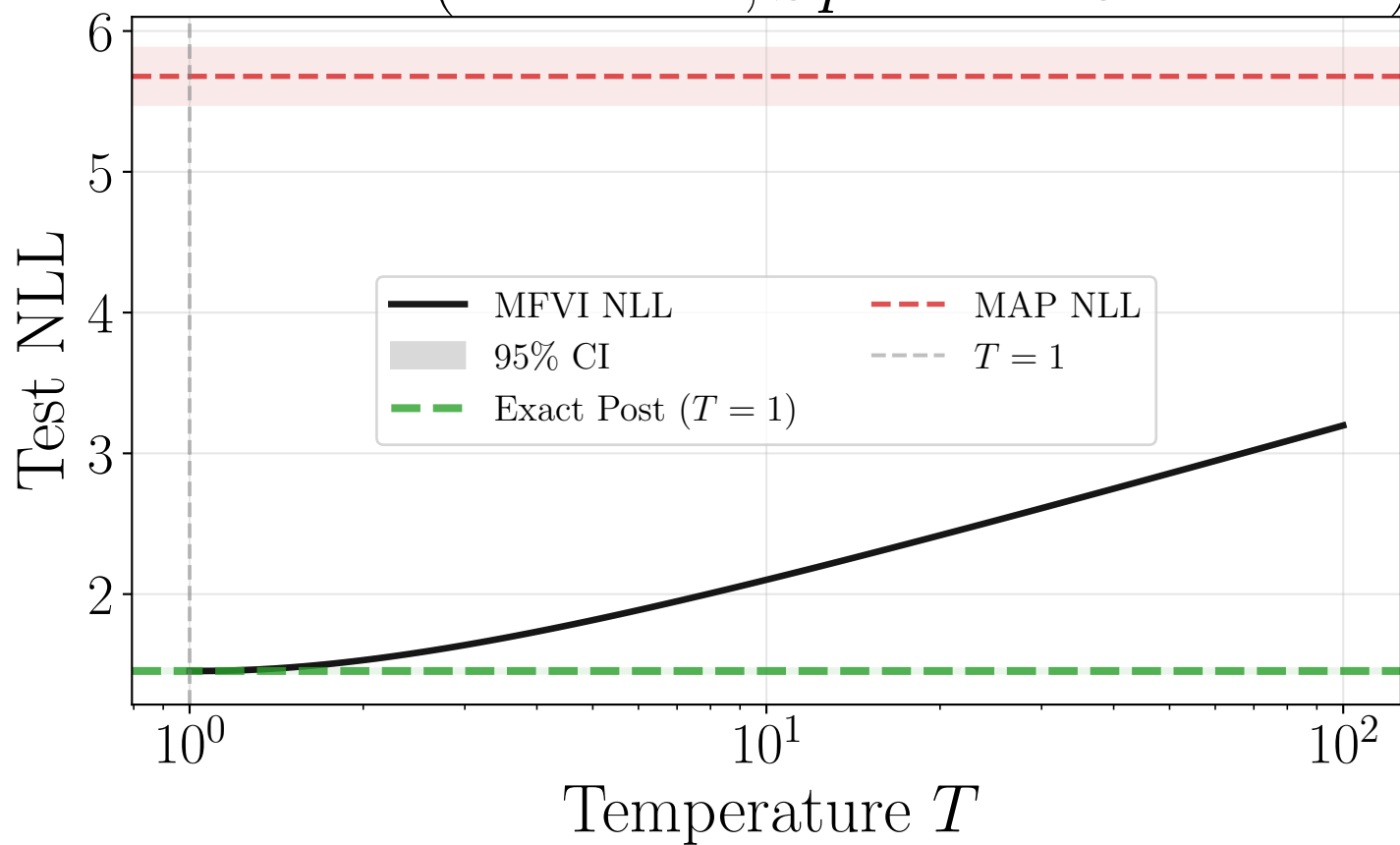
NLL vs T ( P = 1024, SphericalGaussian )
