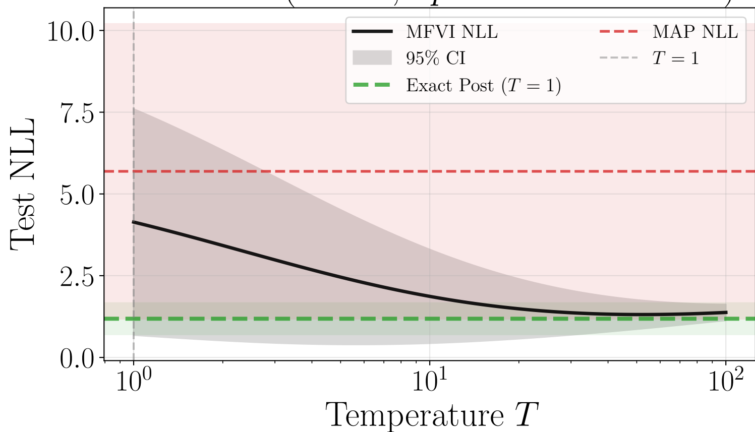
NLL vs T ( P = 1024, SphericalGaussian )
