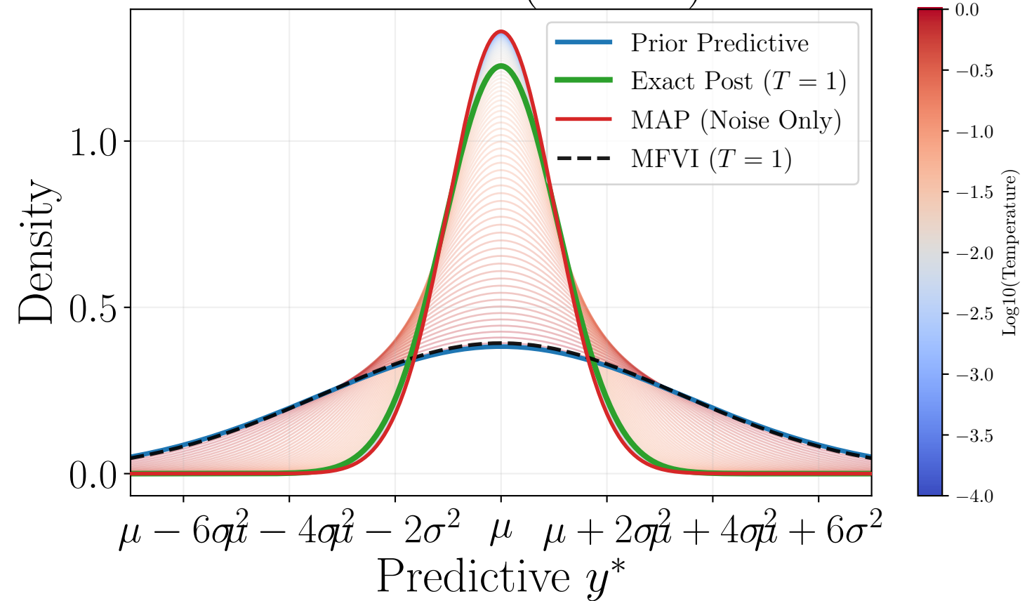
Post Pred ( x^* \propto \mathbf{1} )
