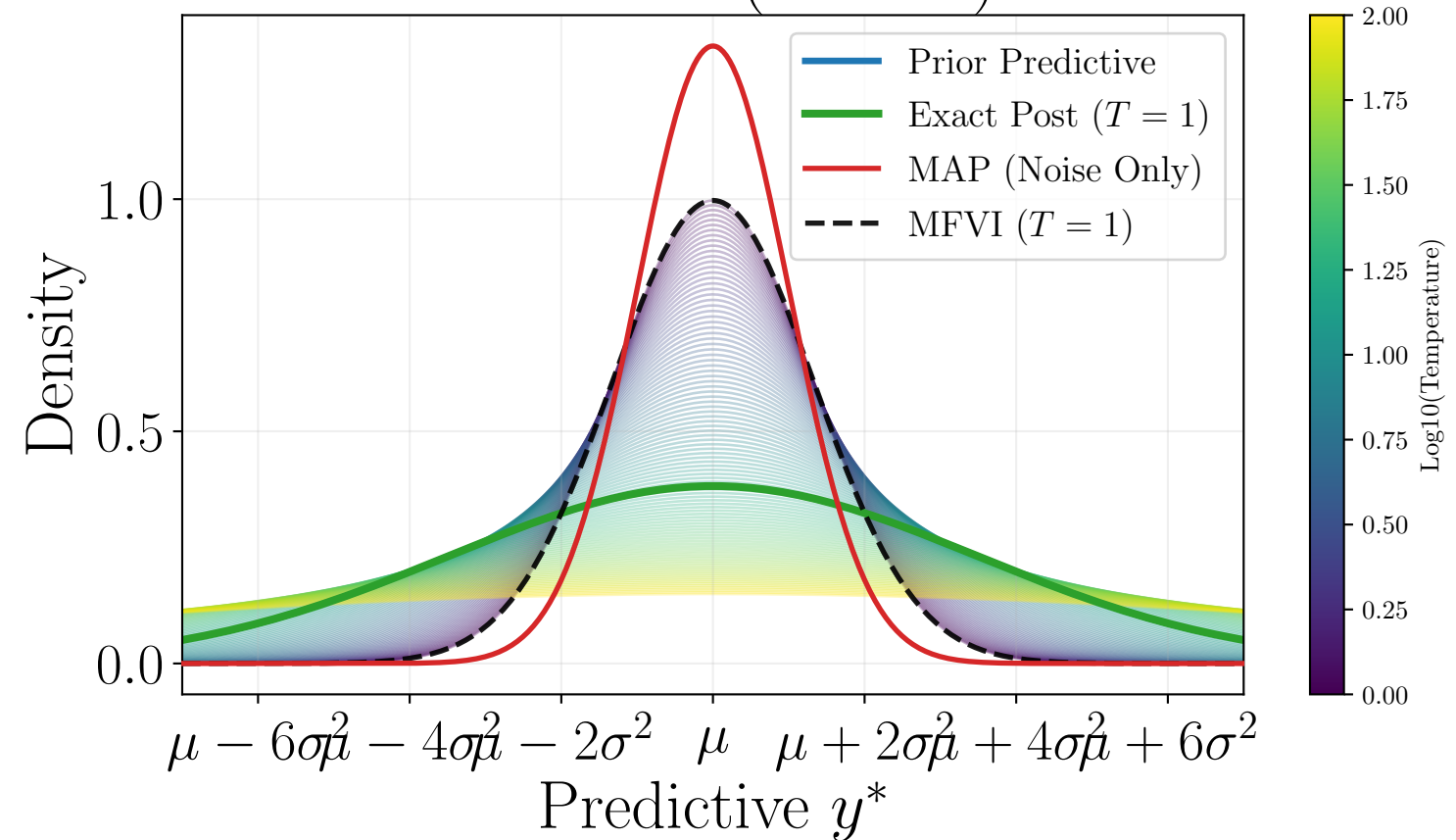
Post Pred ( x^* \perp \mathbf{1} )
