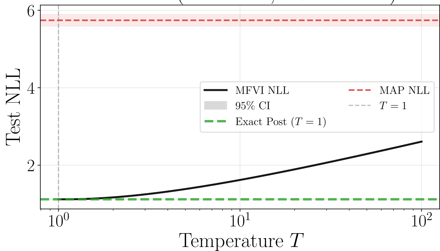
NLL vs T ( P = 1024, OODOrtho )
