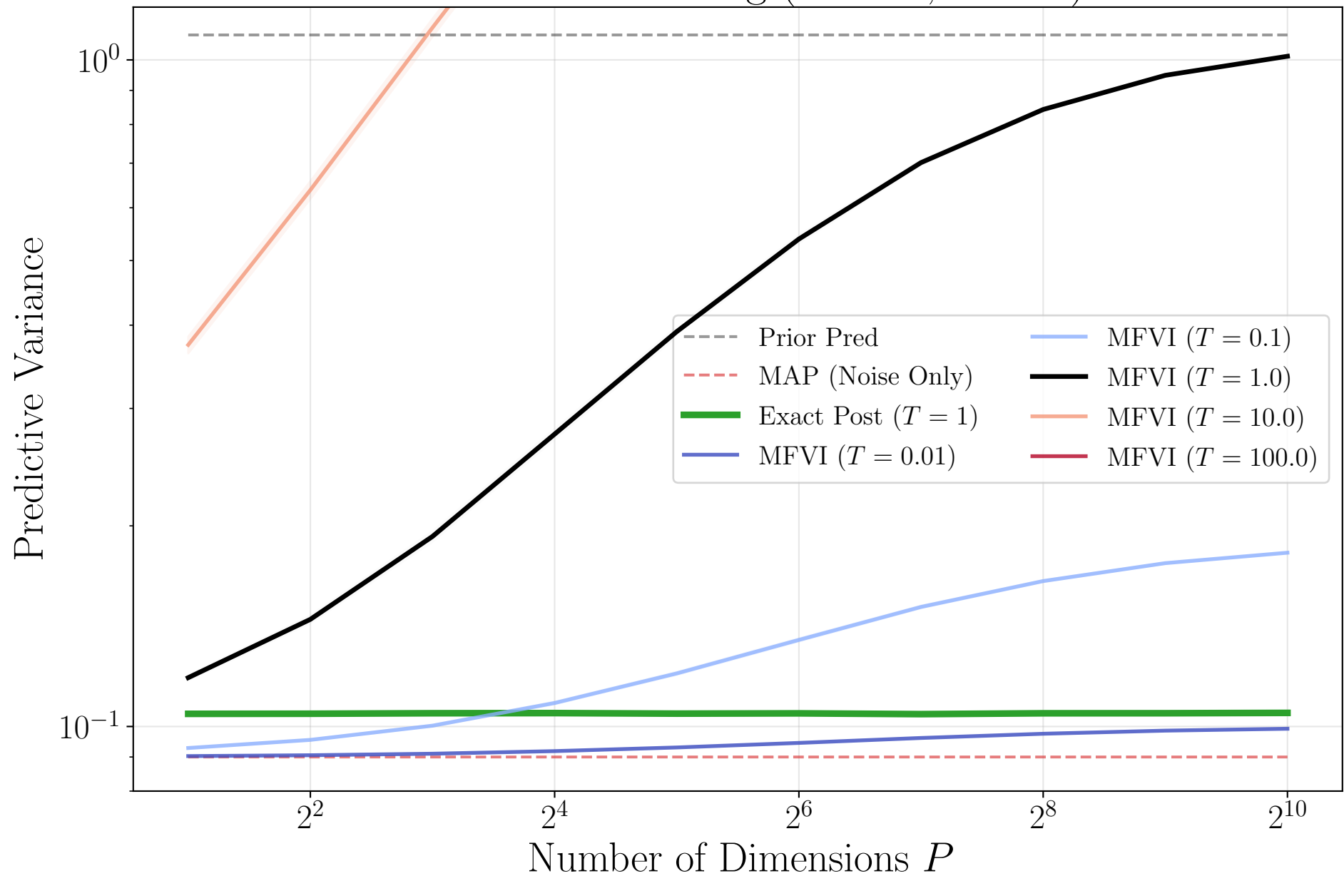
IID Variance Scaling ( x^* \propto \mathbf{1} , N = 8 )
