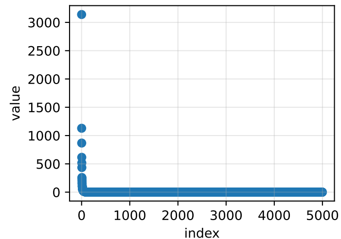
protein
