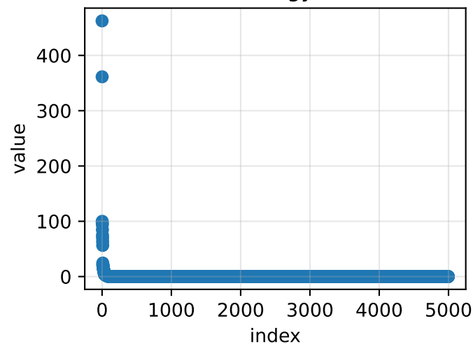
wine
