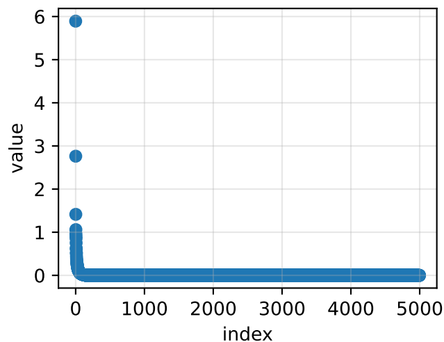
power
