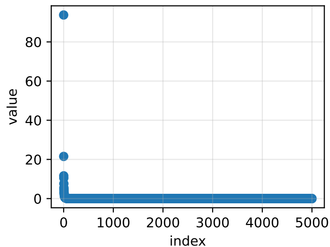
yacht
