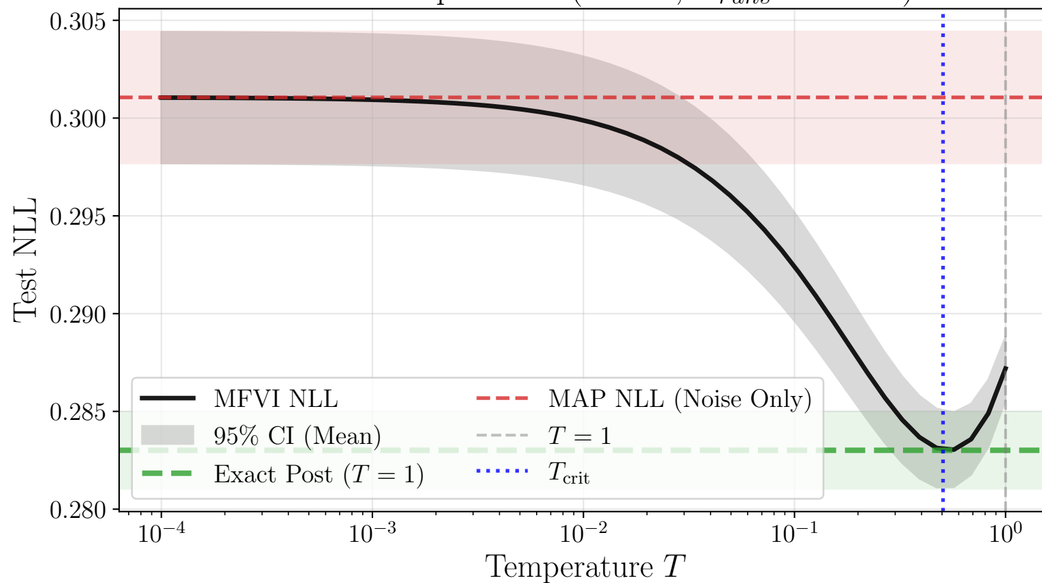
NLL vs Temperature ( P = 2, N_{runs} = 10000 )
