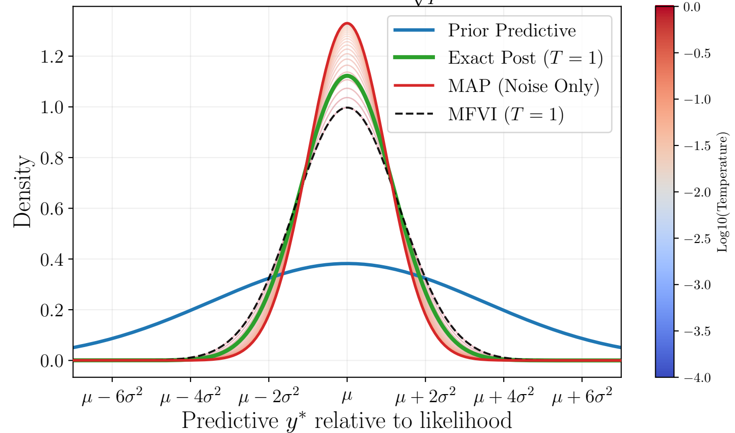
Post Pred ( x^* = \frac{1}{\sqrt{P}}\mathbf{1} )
