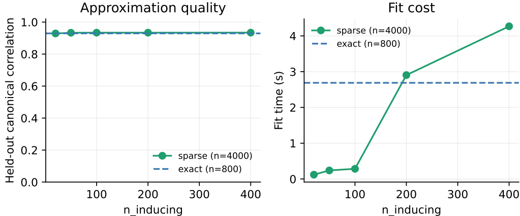
Figure 2: Sparse GaussianProcessCCA on n = 4000 training samples: held-out canonical correlation and fit time as a function of the number of inducing points, against exact inference on a subsample of 800 points (the largest exact fit run for this paper; exact inference is O(n^3) and does not scale to the full 4000-sample training set within a similar compute budget).
