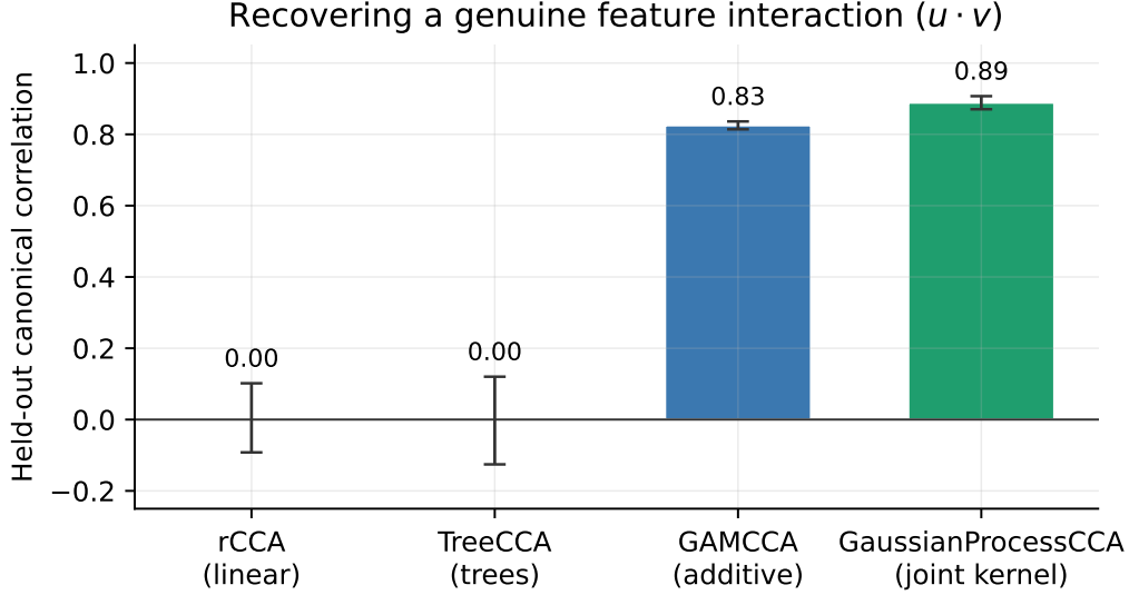
Figure 1: Held-out canonical correlation on the feature-interaction task (Section 5), mean \pm one standard deviation over 10 seeds. GaussianProcessCCA ’s joint, non-additive kernel recovers the signed uv interaction most fully; additive GAMCCA recovers only a partial, sign-blind proxy; linear rCCA and default-settings TreeCCA recover essentially nothing.
