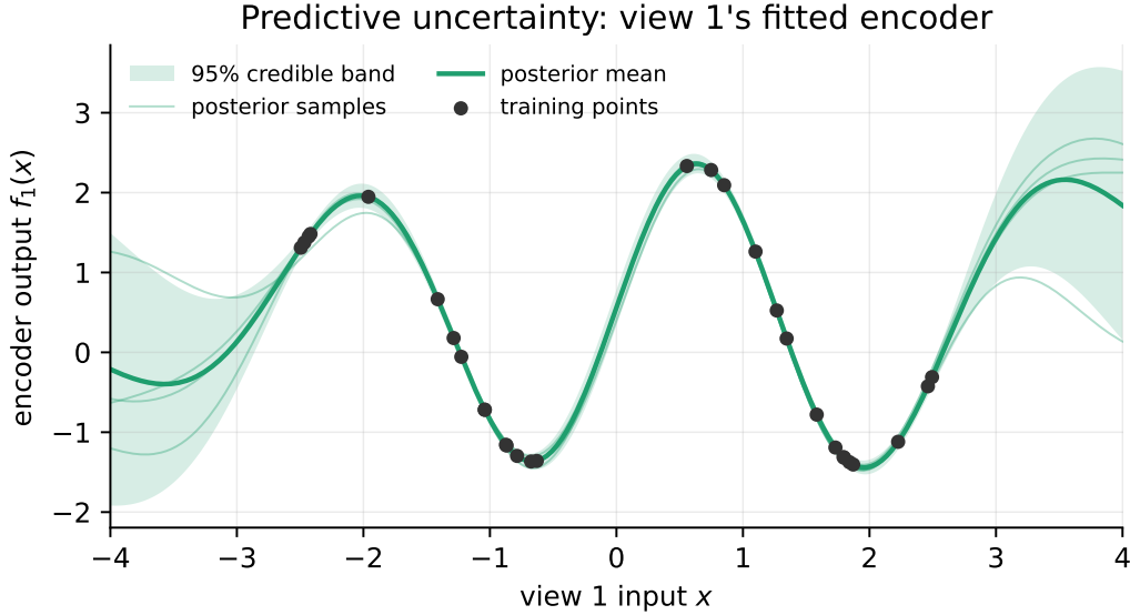
Figure 3: View 1’s fitted encoder on the synthetic x/\sin(2.5x) task: posterior mean, 95% credible band, four posterior sample paths, and the training points’ own projected values. The band and sample paths stay tight near the two training clusters ( x \in [-2.5, -0.5] \cup [0.5, 2.5] ) and flare up beyond them, exactly like the familiar one-dimensional GP regression plot.
