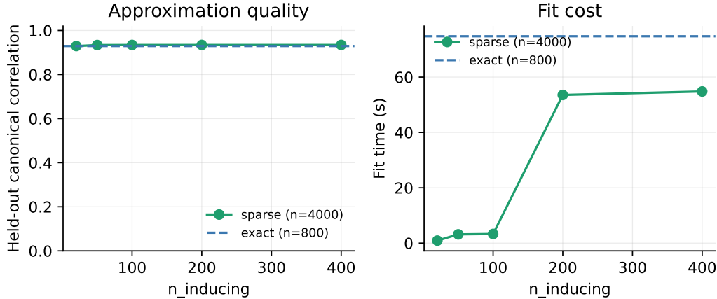
Figure 2: Sparse GaussianProcessCCA on n = 4000 training samples: held-out canonical correlation and fit time as a function of the number of inducing points, against exact inference on a subsample of 800 points (the largest exact fit run for this paper; exact inference is O(n^3) and does not scale to the full 4000-sample training set within a similar compute budget).
