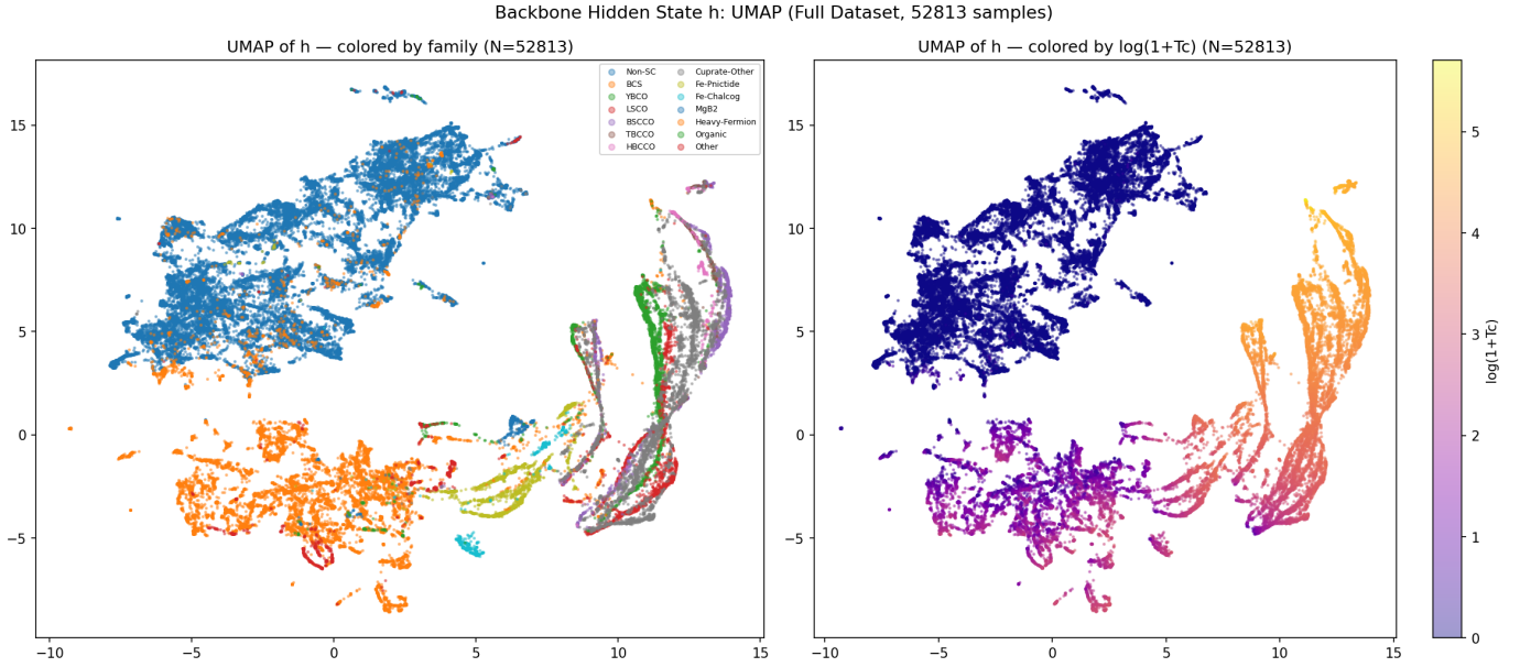
Fig. 2. UMAP of backbone hidden state h[576] for 52,813 samples. Left: colored by superconductor family (14 classes). Right: colored by \log(1 + T_c) . Families form elongated filamentary manifolds with continuous T_c gradients. Cuprate sub-families are clearly separated. The BCS cluster (orange, bottom-left) and non-SC region (blue, top) are well-isolated.
