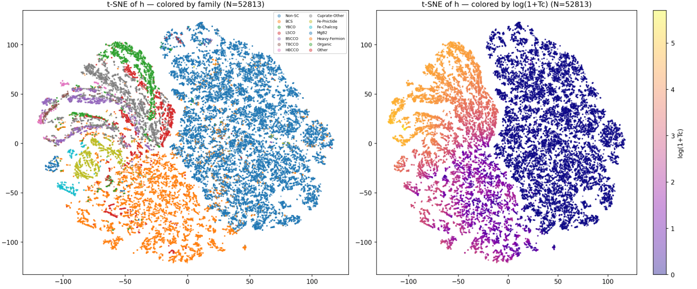
Backbone Hidden State h : t-SNE (Full Dataset, 52813 samples)
