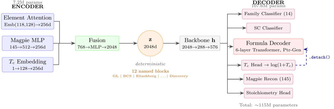
Fig. 1. MAGE architecture. Three encoder branches (element composition, Magpie features, T_c ) fuse into a 2048-dimensional deterministic latent vector \mathbf{z} , partitioned into 12 named physics coordinate blocks. The shared backbone \mathbf{h} [576] feeds six decoder heads. The T_c head conditions the formula decoder via cross-attention memory tokens with .detach() (dashed), creating dual supervision without gradient leakage. Total: \sim 115\text{M} parameters (7.2M encoder, 107.6M decoder).
