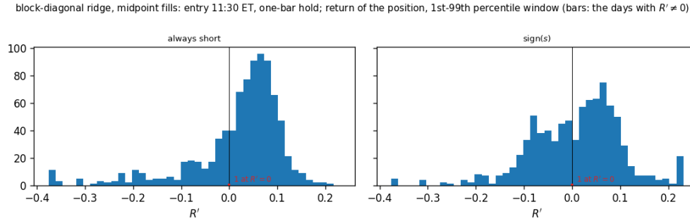
Distribution of the return of the position taken at 11:30 ET, block-diagonal ridge forecast, one panel per rule (returns inside their 1st–99th percentile window).
