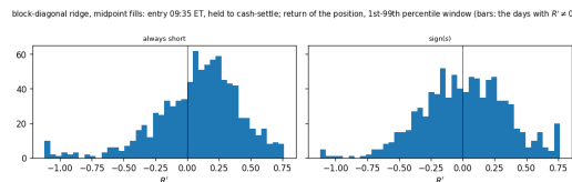
Distribution of the return of the position taken at 09:35 ET, block-diagonal ridge forecast, one panel per rule (returns inside their 1st–99th percentile window).
