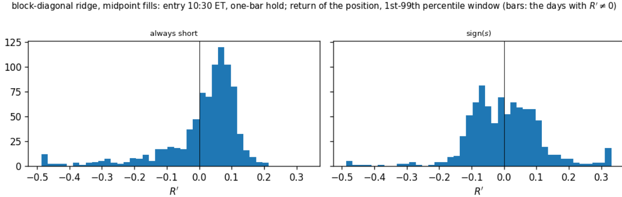
Distribution of the return of the position taken at 10:30 ET, block-diagonal ridge forecast, one panel per rule (returns inside their 1st–99th percentile window).
