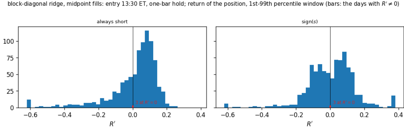
Distribution of the return of the position taken at 13:30 ET, block-diagonal ridge forecast, one panel per rule (returns inside their 1st–99th percentile window).
