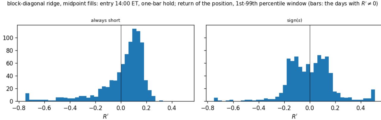
Distribution of the return of the position taken at 14:00 ET, block-diagonal ridge forecast, one panel per rule (returns inside their 1st–99th percentile window).
