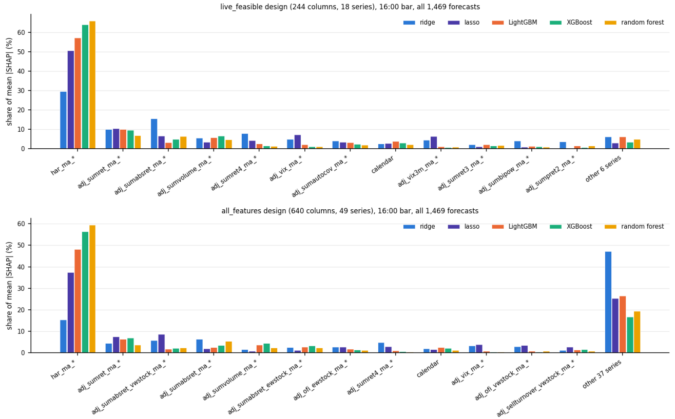
Figure 8: Share of mean |SHAP| by series, one bar per model (all forecasts of the 16:00 bar). Top: live-feasible design (Table above). Bottom: the all-features design (640 columns, 49 series), the 12 largest series and the rest summed. LGBM = LightGBM, XGB = XGBoost, RF = random forest.
