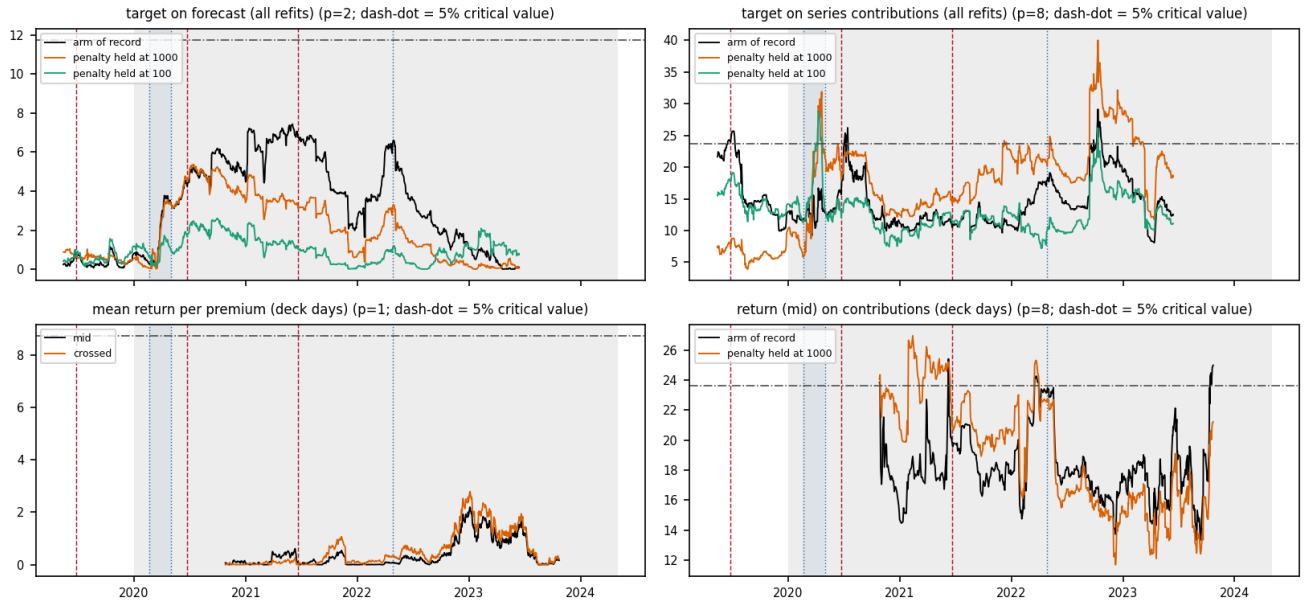
Figure 5: Wald statistic for a break at each date (the sup-Wald scan) with its 5% critical value. Vertical lines as in Figure 4.
