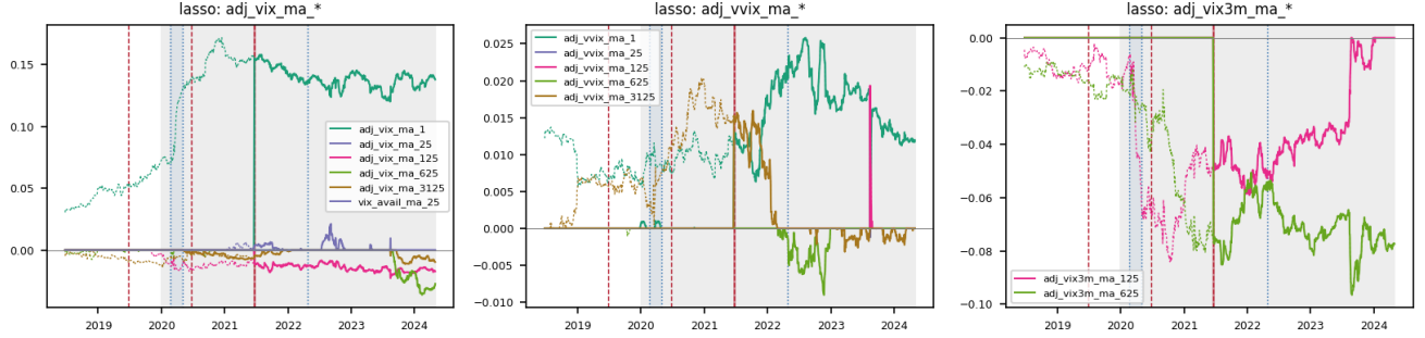
Figure 7: The lasso's standardized weights on the VIX-family columns (design column names; colour = lag as in Figure 1): solid = lasso of record, dashed = penalty held at 0.001 from the start. Thick red line = the lasso's penalty re-choice; other lines as in Figure 4. Only columns the lasso of record ever keeps are drawn.
