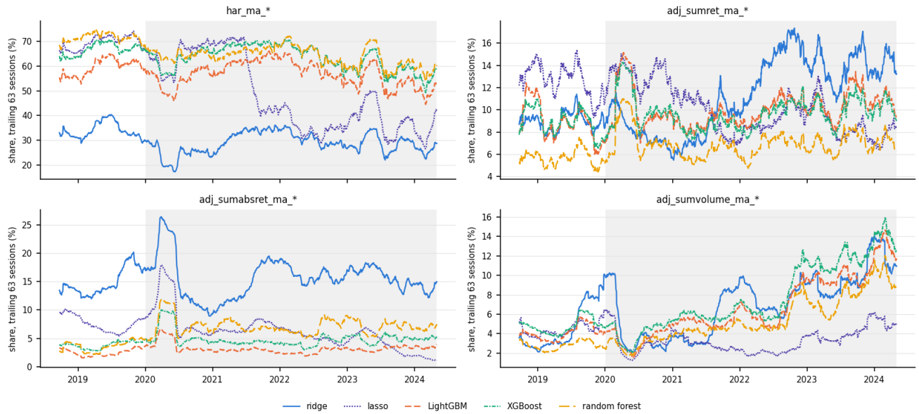
Figure 9: Share of mean |SHAP| over a trailing 63-session window for the four largest series, every model (the trees’ SHAP values are per forecast, so the share can be followed over time like the ridge’s in Section 2). Grey = the deck period.
