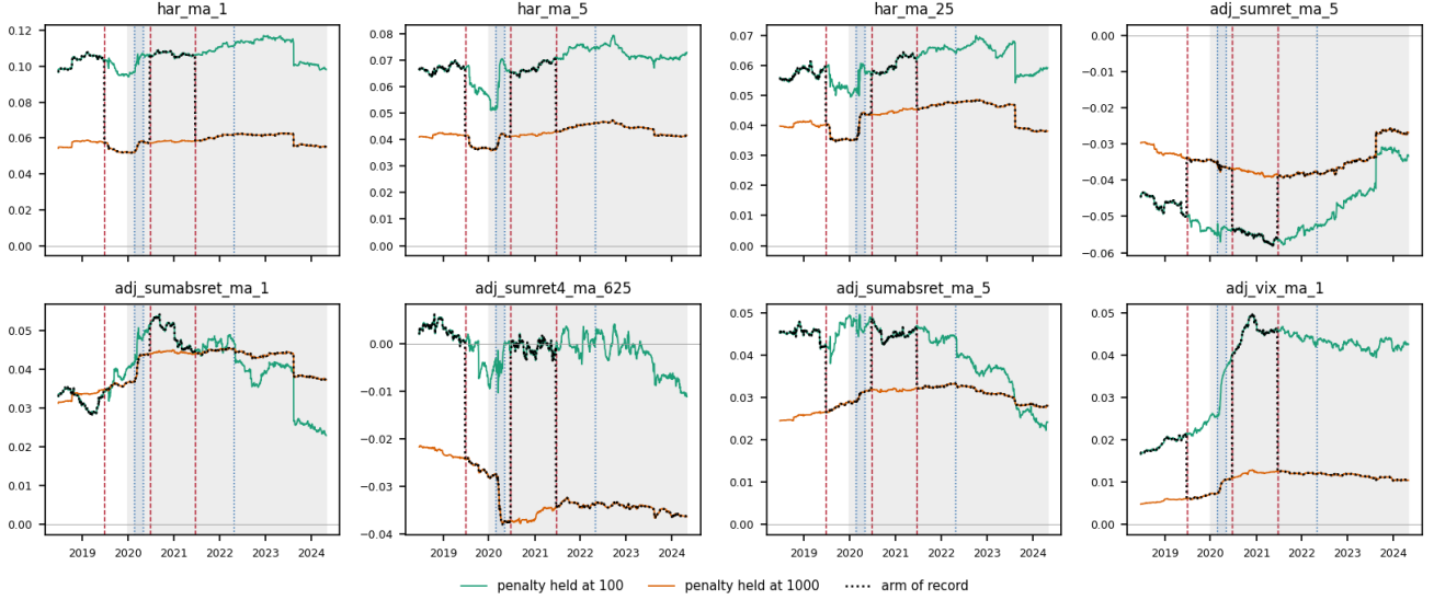
Figure 4: Standardized weights of the eight largest inputs (design column names, key under Figure 1): the arm of record (dotted black) and the same arm with the penalty held at 100 (green) or 1000 (orange). Red dashed = penalty switches; blue dotted = COVID start/end and every-day expirations; blue band = Feb–Apr 2020; grey = deck days.
