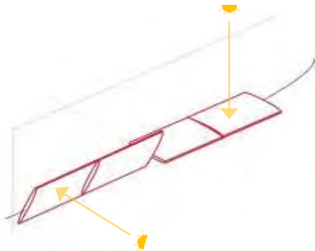
Solar shading System responsive to sun angle.
