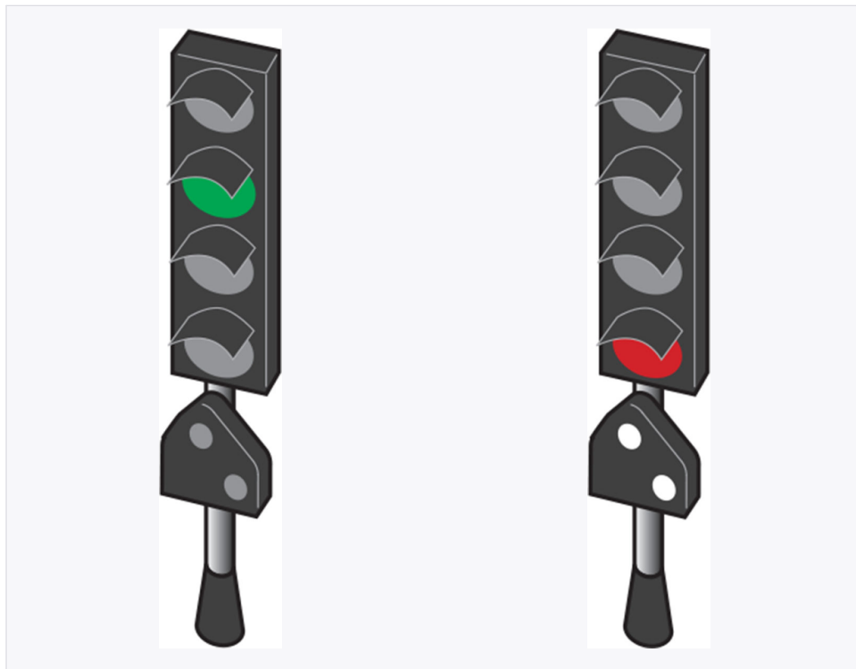
Position-light signal associated with a main aspect — obey the main signal (green, left) — RS521 §2.7
