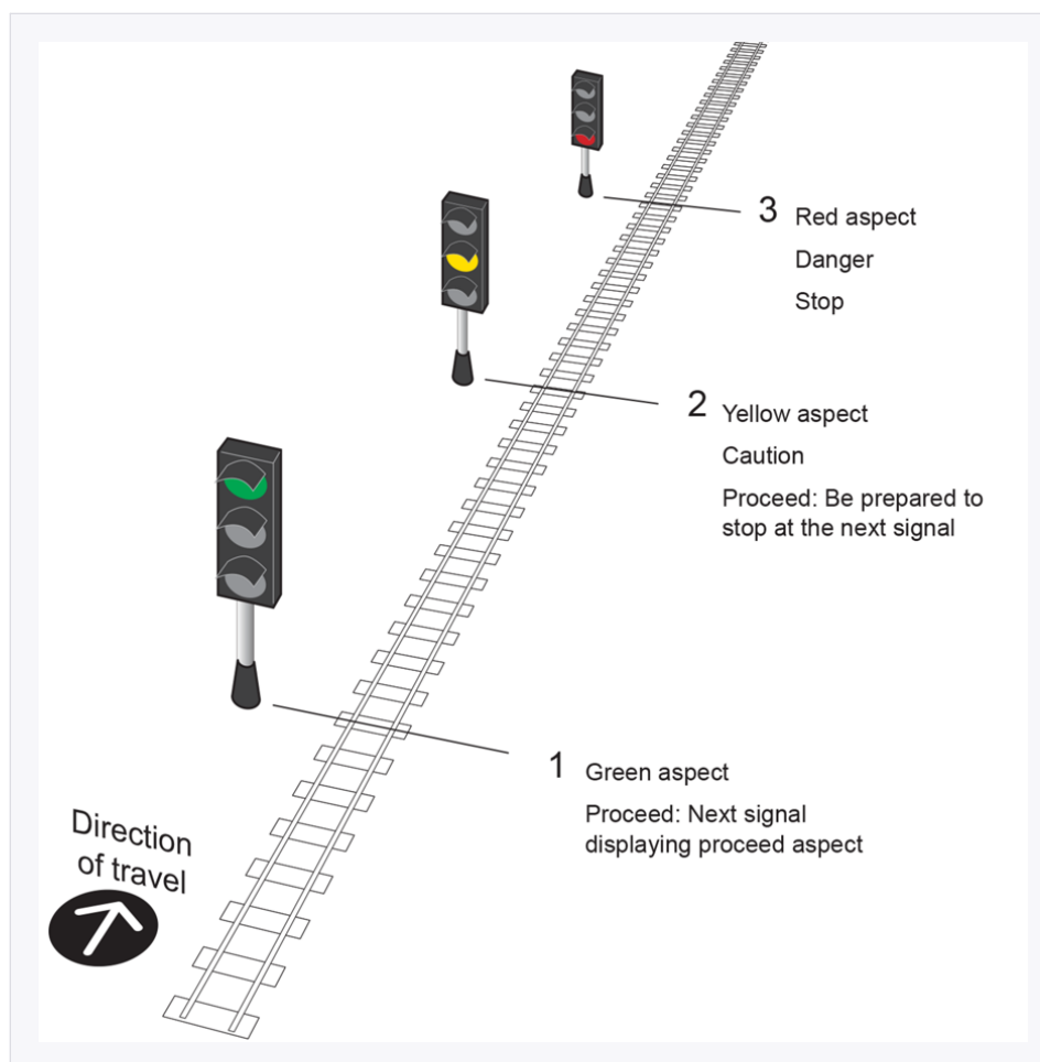
Three-aspect signalling — the normal sequence — RS521 §2.1
