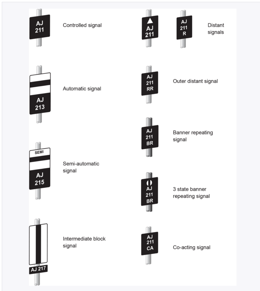
Every identification plate type shown together — RS521 §1.2
