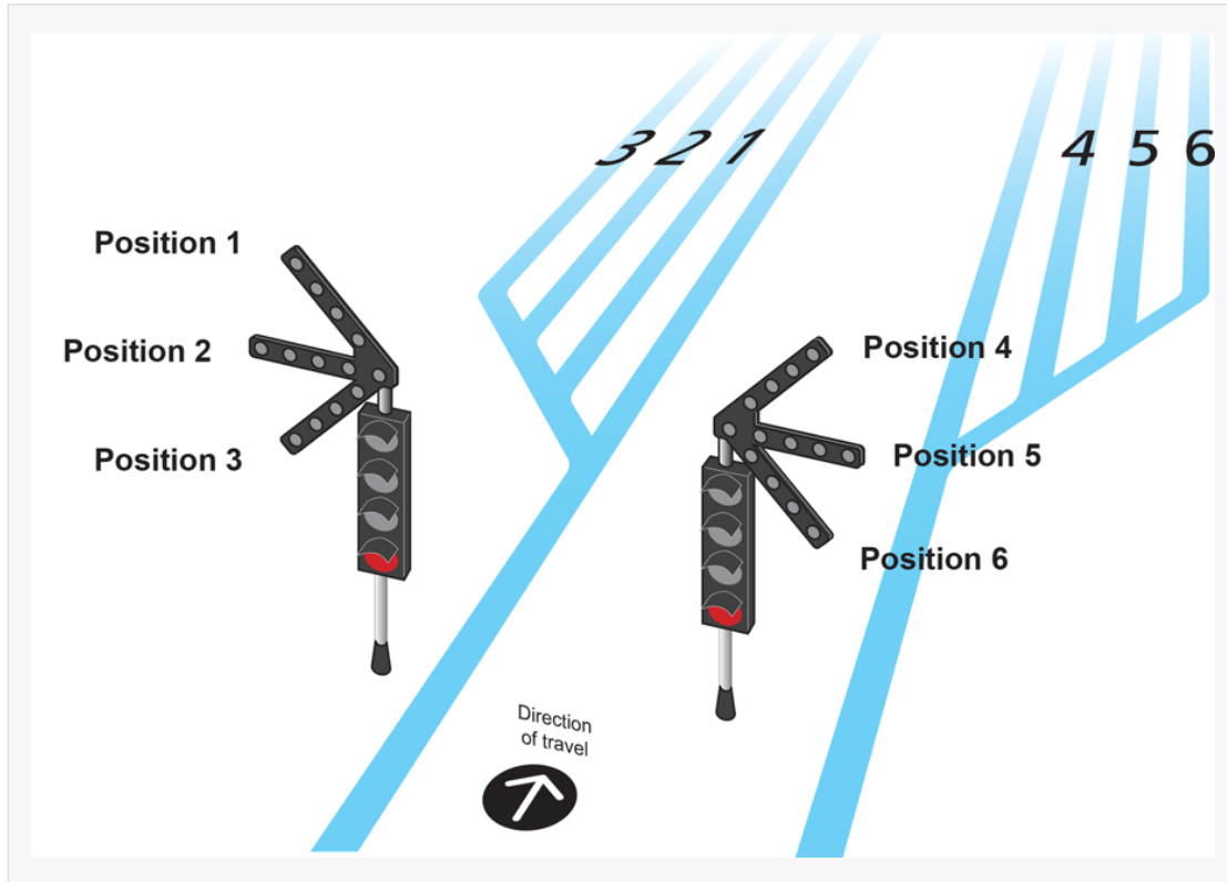
Junction indicator feather positions, both sides of the signal — RS521 §2.3
