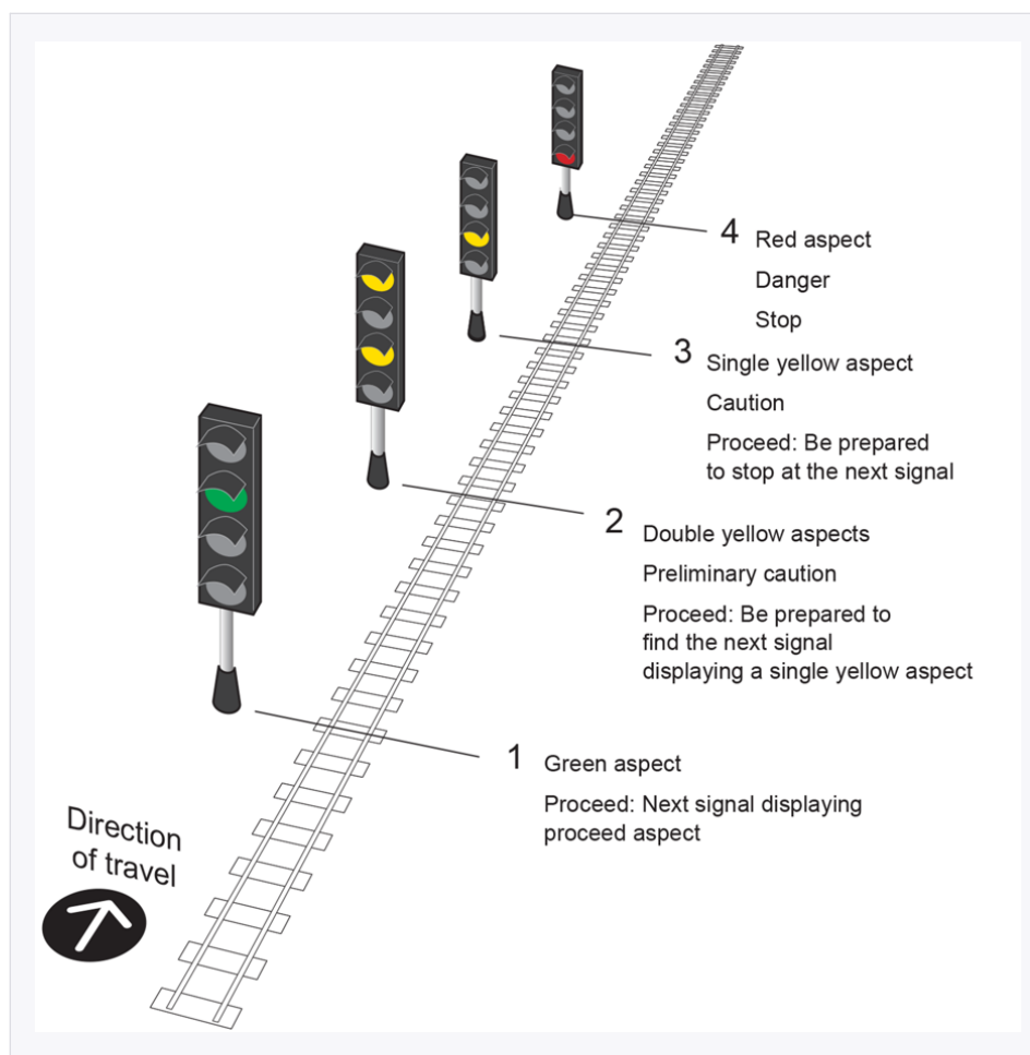
Four-aspect signalling — the normal sequence — RS521 §2.2
