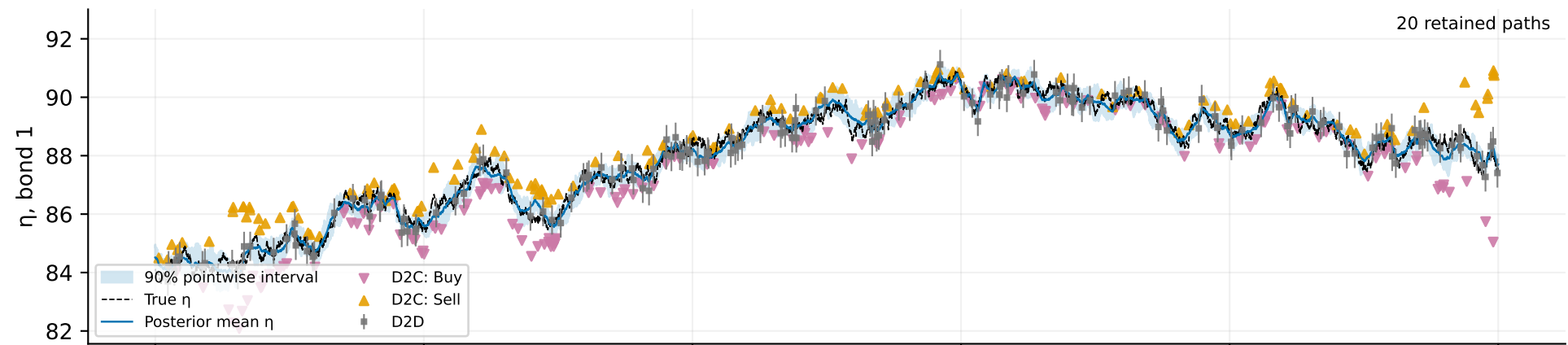
Bootstrap PF
