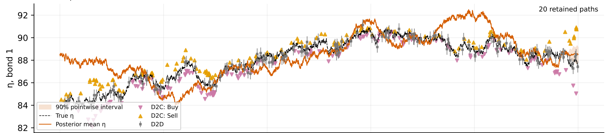
Guided PF
