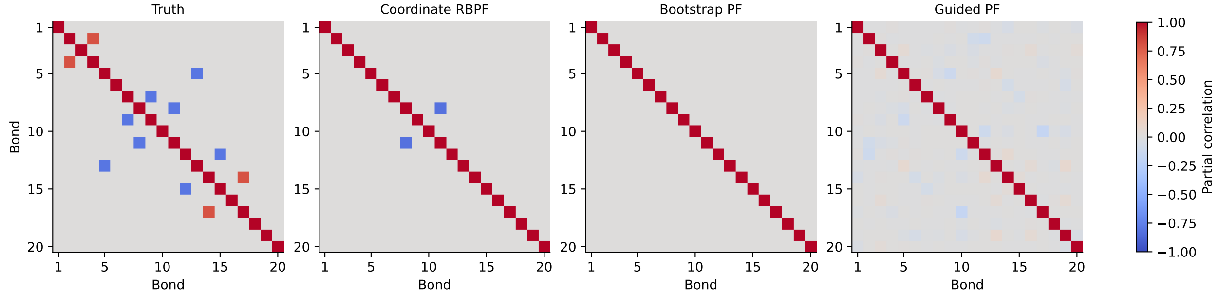
Partial-correlation posterior means; D=20, seed=1234
