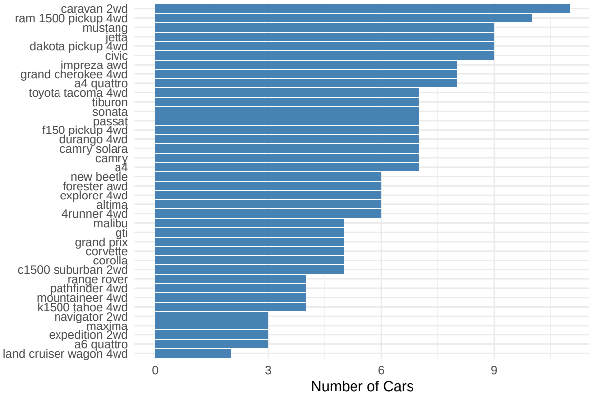
Number of Cars per Model in the MPG Dataset
