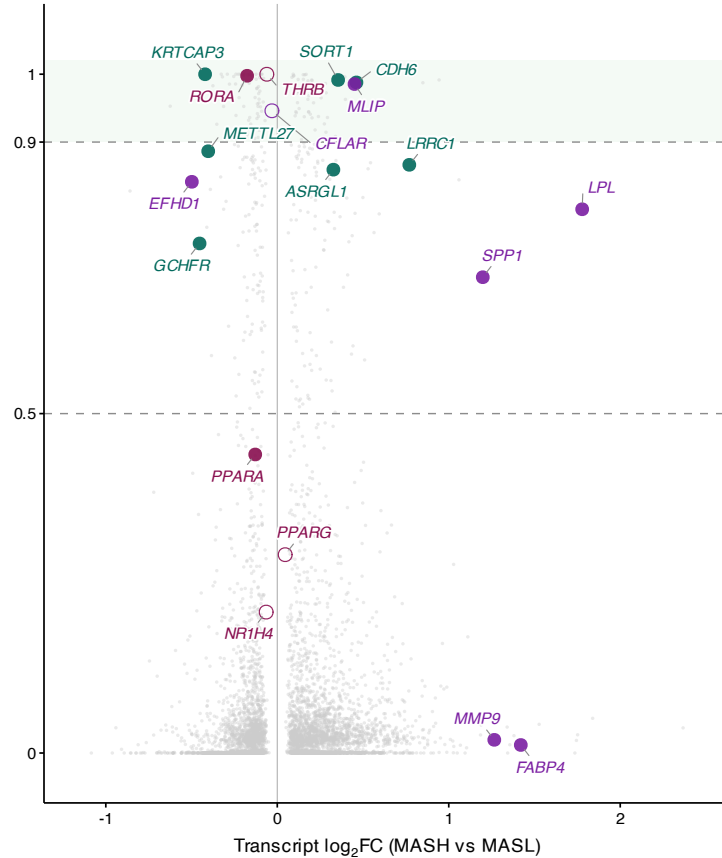
COLOC vs. MASH-vs-MASL DEG
