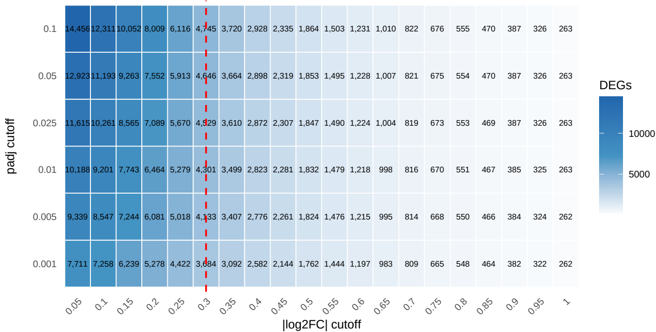
Threshold stability
