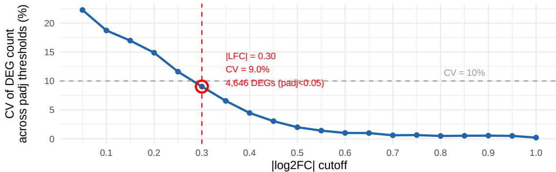
Threshold stability
