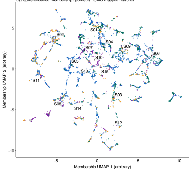
Signature-excluded membership geometry: 5,445 mapped features
