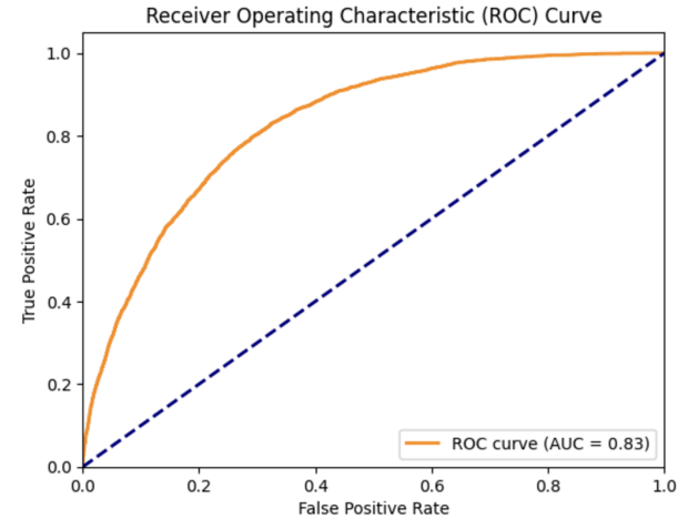
Figure 1. Area Under the Receiver Operating Characteristic Curve of RandomForest Classifier
