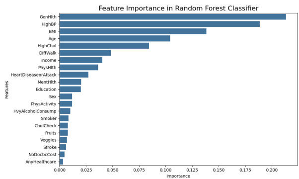
Figure 3. Bar chart of important features in RandomForest Classification
