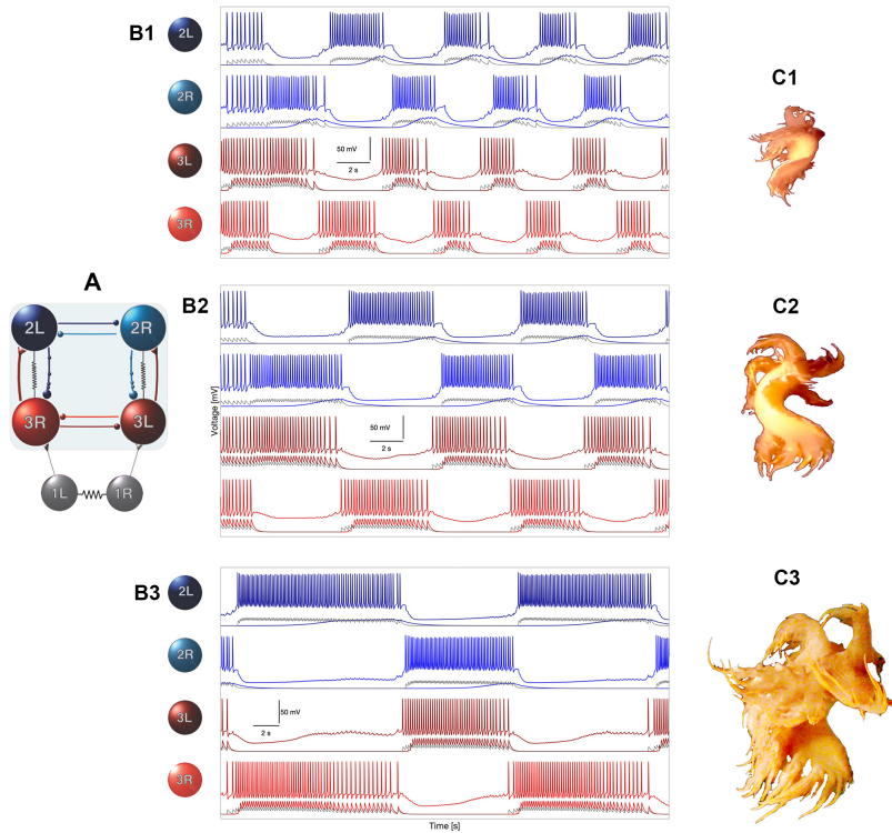
FIG. 3. Developmental scaling of swim dynamics. CPG circuit as it adjusts to the changing body size and biophysical properties of Dendronotus iris throughout development. (A) Schematic of the canonical swim CPG circuitry composed of the four core interneurons – Si2L/R and Si3L/R – organized into two bilaterally symmetric inhibitory–excitatory modules. These twisted pairwise modules, interconnected by diagonal excitatory and reciprocal inhibitory synapses, form the structural basis for anti-phase left–right alternation and network-level rhythmogenesis. (B) Representative traces showing the voltage waveforms (top) and corresponding neurotransmitter release probabilities (lower traces) for the four core interneurons (SiN). These patterns are driven by tonic excitatory input from the Si1 interneurons, which provide the initiating drive necessary for the onset and termination of rhythmic bursting across the network. The combined electrical and chemical interactions among Si2 and Si3 neurons give rise to a robust, self-sustained oscillatory rhythm that defines the basic swim motor pattern. (C) Developmental scaling of swim rhythm dynamics across the lifespan of Dendronotus iris . As the animal grows from juvenile (approximately 30 g) to adult (approximately 300 g) stages—a tenfold increase in body mass—the swim period correspondingly slows from approximately 2–3 s in juveniles to 12–14 s in mature individuals. Despite this pronounced temporal scaling, the underlying phase relationships among the four CPG interneurons remain invariant, as reflected in the voltage traces shown in panel B. This remarkable stability demonstrates the CPG’s capacity for self-similar temporal rescaling, ensuring that locomotor coordination and bilateral phase balance are preserved across a broad range of physiological and morphological states. To discuss and compare with Fig. 10 from the aspiring experimental study 13 .
