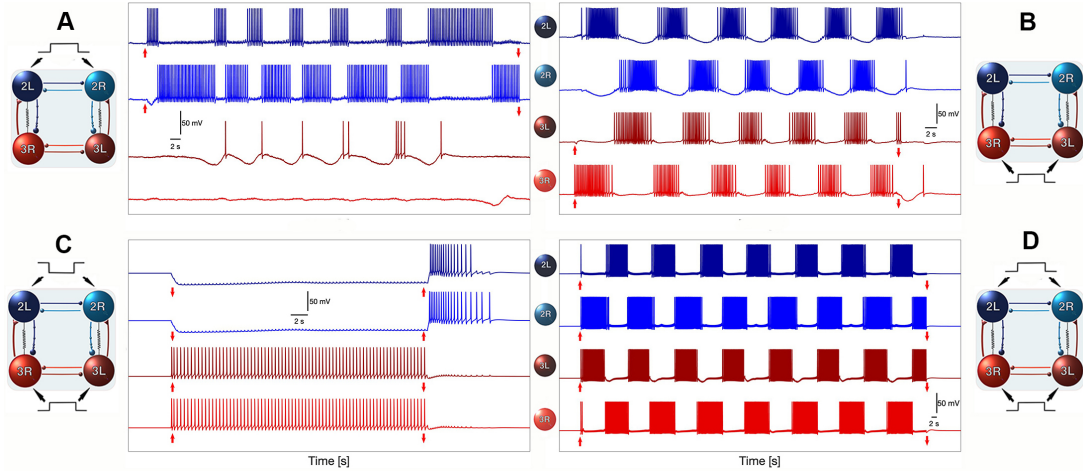
FIG. 6. Symmetric perturbation experiments validating the swim CPG model. Fact-check list II: Compare the four modeling panels with their corresponding experimental originals shown in Figs. 7Ai–Di of Ref. 15 . The swim CPG model exhibits responses during control swims that closely match the biological data under various temporal perturbations—produced by applying hyperpolarizing or depolarizing current pulses (red vertical arrows) to targeted interneurons—thereby validating the model against its experimental counterparts. These results confirm that the modeled CPG reproduces the timing, polarity, and recovery dynamics of the living network across a range of perturbation strengths.
