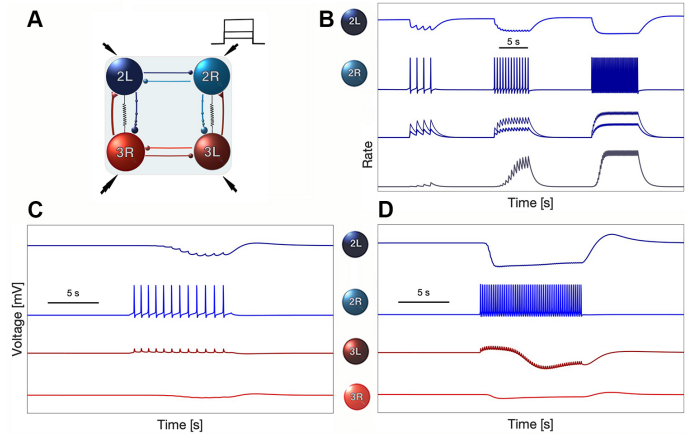
FIG. 1. Calibration of two synaptic models, \alpha and logistic, and validation of inhibitory coupling mechanisms. Fact-check list I: Compare panels C and D with the corresponding neurophysiological recordings presented in Fig. 7 of Ref. 13 . (A–B) Three positive current pulses of progressively increasing amplitude were applied to Si2R to calibrate the \alpha -synapse and logistic synapse models (bottom trace), as well as to reproduce the inhibitory postsynaptic potential (IPSP) responses observed in the contralateral Si2L (top trace in panel B). (C–D) Two positive current pulses injected into Si2R evoked accumulating IPSP responses in Si2L (top trace) and elicited both fast and slow echo responses in Si3L. These echoes arise from distinct mechanisms: a fast component mediated by the electrical coupling and a slower, delayed inhibitory response mediated by the logistic synapse between Si2R and Si3L. Together, these features reproduce the experimentally observed dynamics and confirm the functional roles of electrical and chemical inhibition within the swim CPG circuitry (see Fig. 2A).
