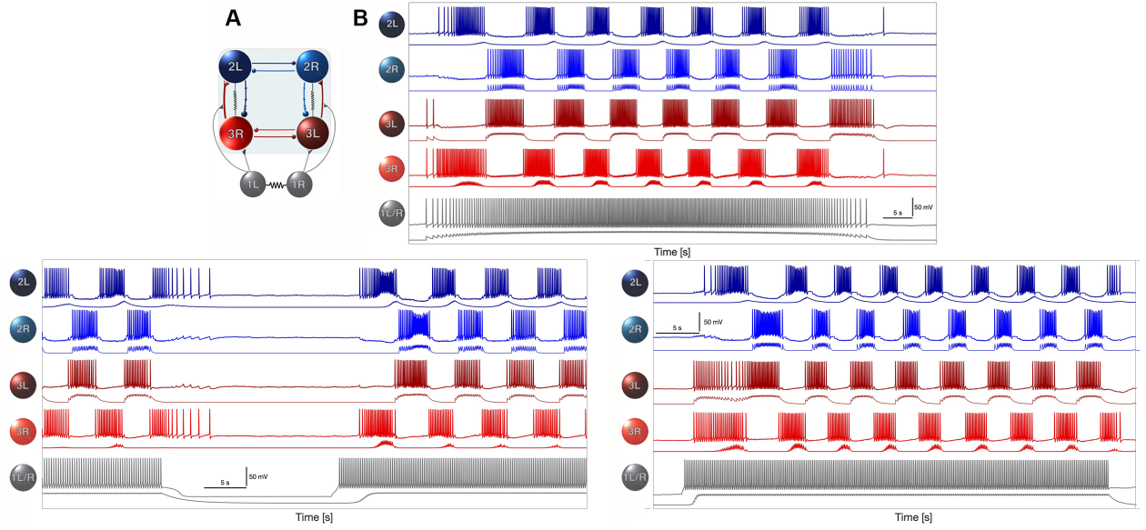
FIG. 7. Role of Si1–Si3 interactions in rhythmogenesis, episode control, and network resilience. Compare the modeling results with their experimental counterparts in Ref. 2 : panel A corresponds to Fig. 2A, and panels B and C correspond to Figs. 3A and 3B, respectively. (A) Swim CPG circuitry in which Si1 neurons provide excitatory drive to both Si3 neurons and regulate neuromodulation in the excitatory Si3→Si2 synapses. (B) Gradually increasing depolarizing drive from Si1 activates the Si3 neurons, thereby gradually initiating and subsequently terminating the rhythmic bursting that defines the swim CPG; in the absence of neuromodulatory input, this Si1→Si3 pathway alone can sustain transient rhythmic activity across the core network. (C) Abrupt hyperpolarization of the Si1 neurons halts rhythmicogenesis, leading to immediate cessation of oscillatory activity; upon release from this perturbation, the CPG rapidly recovers and resumes coordinated bursting, demonstrating its intrinsic resilience and built-in reassembling capacity. Fast Si1 depolarization followed by later hyperpolarizing pulses triggers, maintains, and eventually terminates a swim episode in the CPG circuit. Shown underneath the voltage waveforms are simulated neurotransmitter release probabilities using the synaptic \alpha -model (red for excitatory connections Si3s→Si2s; grey for excitatory connections Si1s→Si3s; light blue for reciprocal inhibition between Si2s and between Si3s) and logistic model (dark blue for inhibitory connections Si2s→Si3s) for the fast and slow chemical synapses, respectively.
