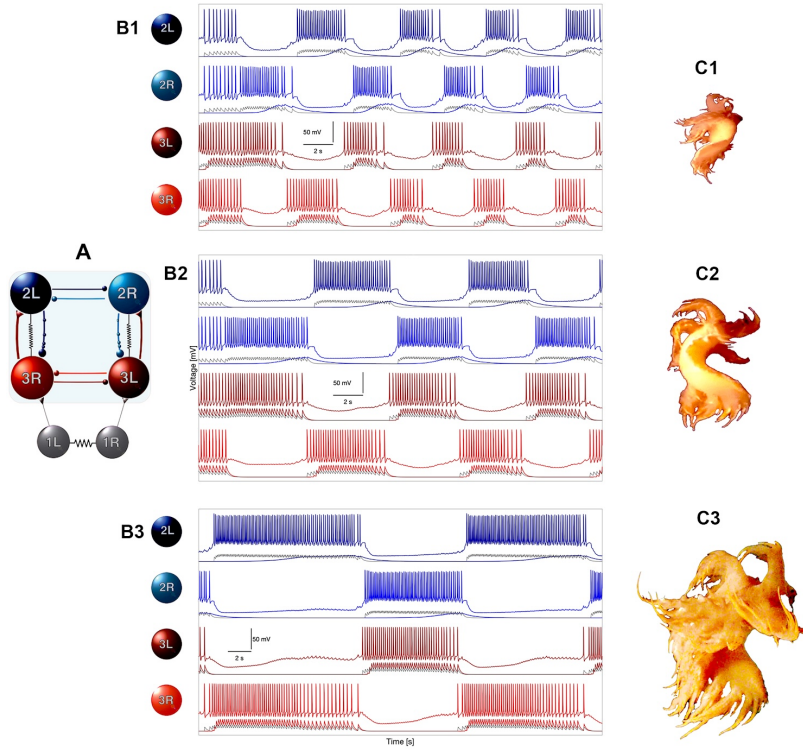
FIG. 1. Circuit schematic and model-derived hypothesis for frequency adaptability in the Dendronotus iris swim CPG. The four-cell circuit assembles excitatory-inhibitory loops together with two contralateral half-center oscillators into a network that reliably produces left-right alternating bursts. Although the constituent subcircuits are nearly oscillatory on their own, the full network is robust, and its burst frequency can be tuned by changing the kinetics of a single symmetric pair of synapses.
