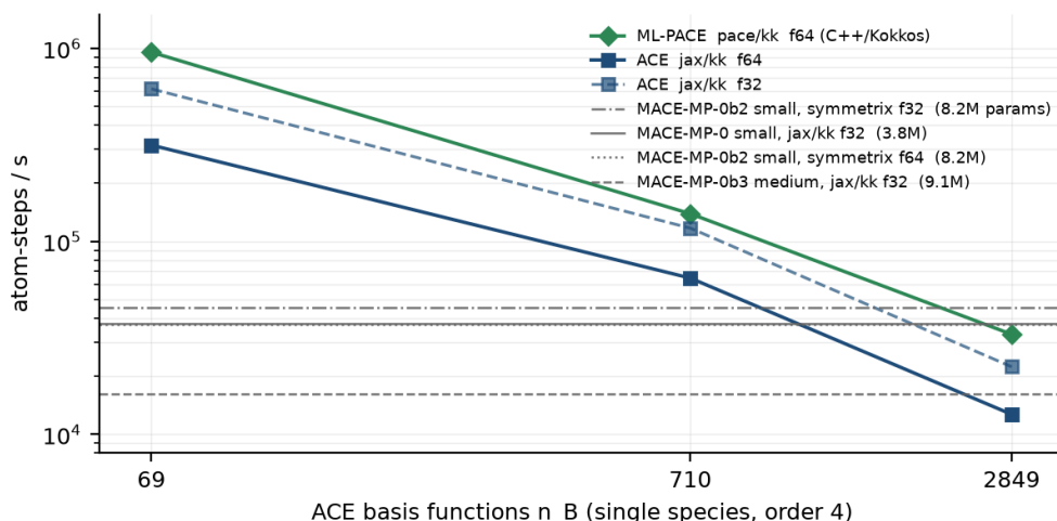
Figure 4: LAMMPS throughput at 1 728 Si atoms, one rank, one RTX A4500 (moriarty). ACE through pair_style jax/kk at three basis sizes (order 4, lmax 4–5, cutoff 6 Å), ML-PACE pace/kk at matched basis shape (78 / 693 / 2 874 functions, 0.9–13% off ours), and three MACE foundation models through jax/kk (lammps-jax) or symmetrix (hand-written Kokkos). Every engine was gated against the others before timing: ACE jax/kk vs Python 1e-13 eV/Å; symmetrix vs jax/kk on the same MACE checkpoint 4e-5 eV/Å.
