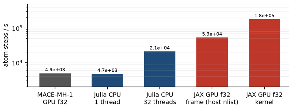
Figure 3: Throughput of the degree-6 d \leq 16 student on one host (lestrade: 32 cores, RTX 4000 Ada), 256–384-atom cells. The JAX kernel runs 32–38 \times the teacher; a single Julia core matches the teacher on a GPU.
