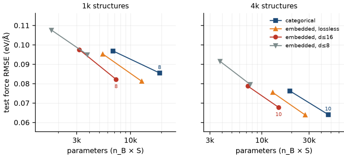
Figure 1: Test force RMSE against parameter count (corrected model). Point labels are the polynomial degree. The embedded lossless model tracks or beats the categorical one at every degree with 1.3–1.7× fewer parameters; d \leq 16 sits within 1–6% at 2.1–3.2× fewer.
