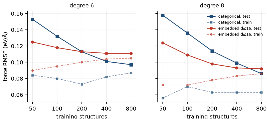
Figure 2: Learning curves on the 1k set (test solid, train dashed), measured with the pre-correction embedded model ; the corrected curves are being re-run. Degree 6 is basis-limited for both models; at degree 8 the categorical model is still data-limited (gap 0.022 at N = 800 ) while the embedded one had converged.
