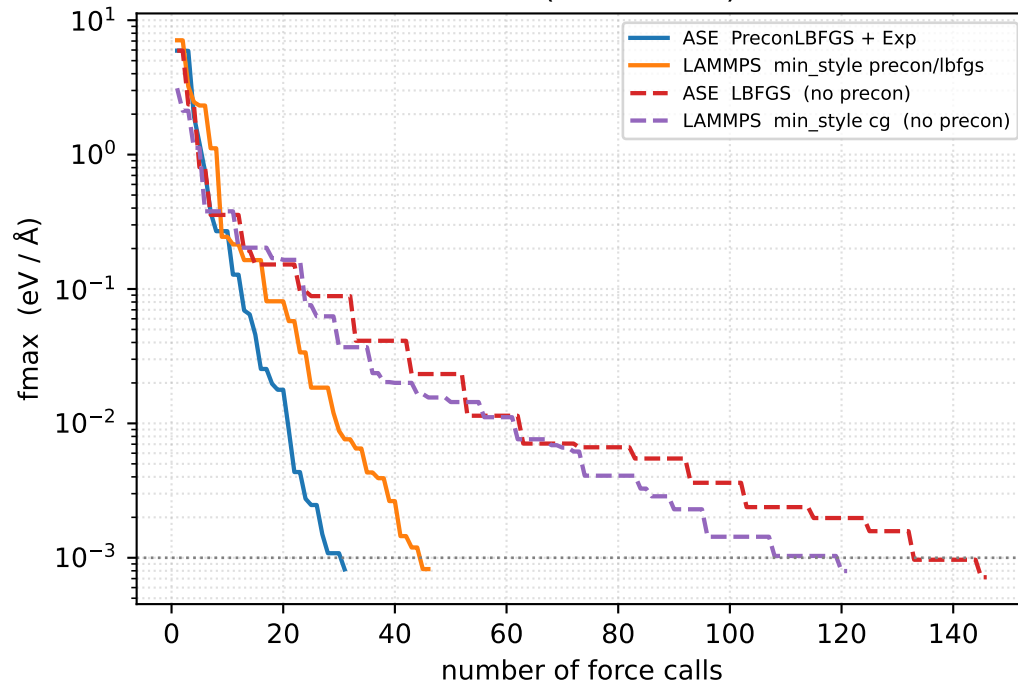
iceVIII (432 atoms)
