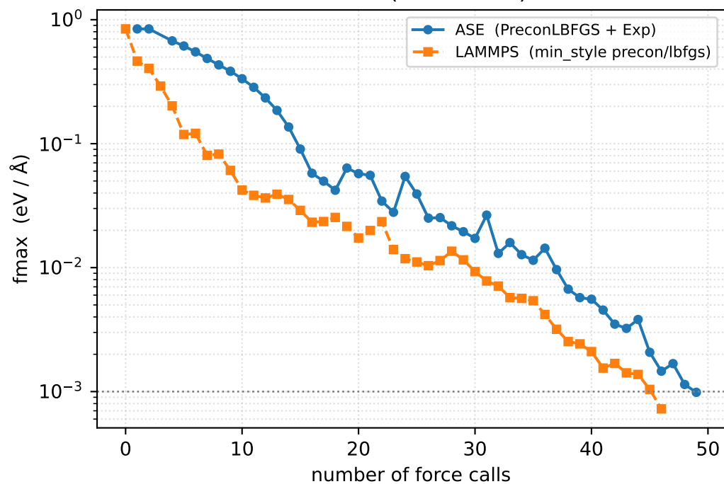
iceVIII (432 atoms)
