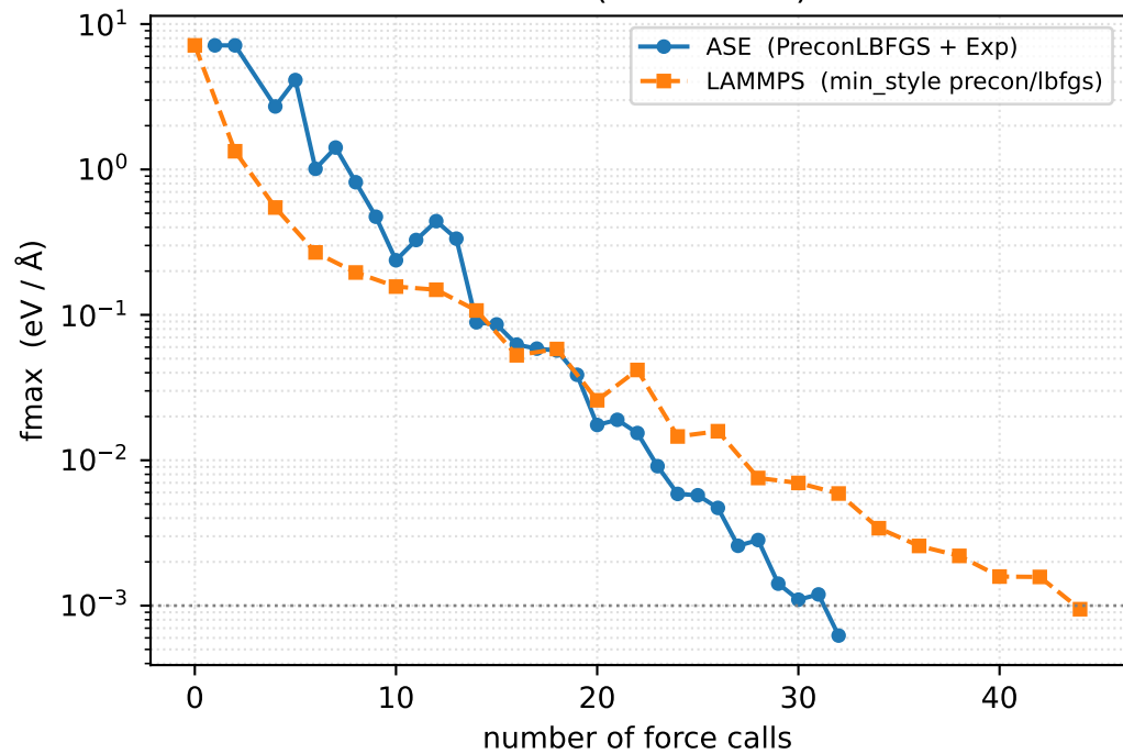
iceVIII (432 atoms)
