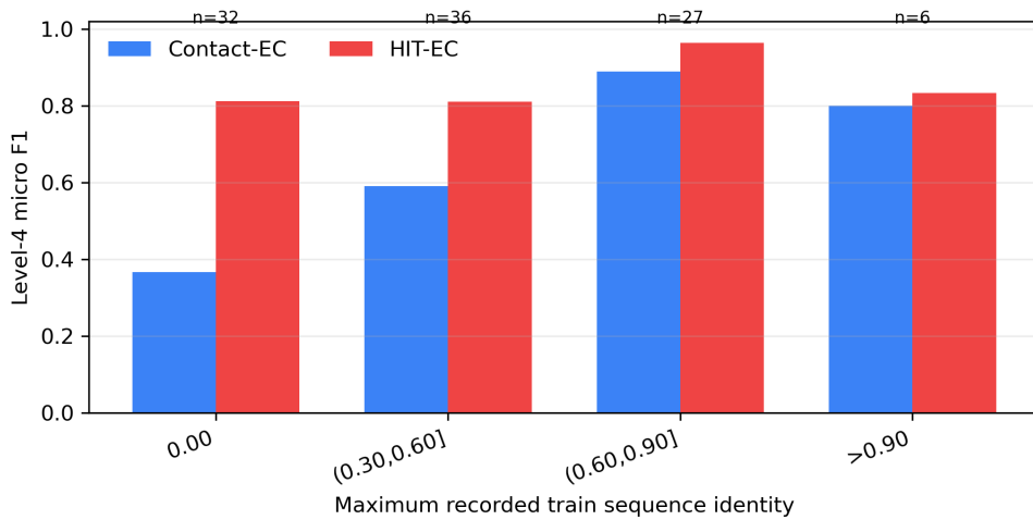
Figure 5: Level-4 micro F1 by maximum recorded train-set sequence identity on the 101 temporal proteins with available EC-Bench similarity metadata. The result motivates future Foldseek/TM-align or CATH/SCOP fold-disjoint testing.
