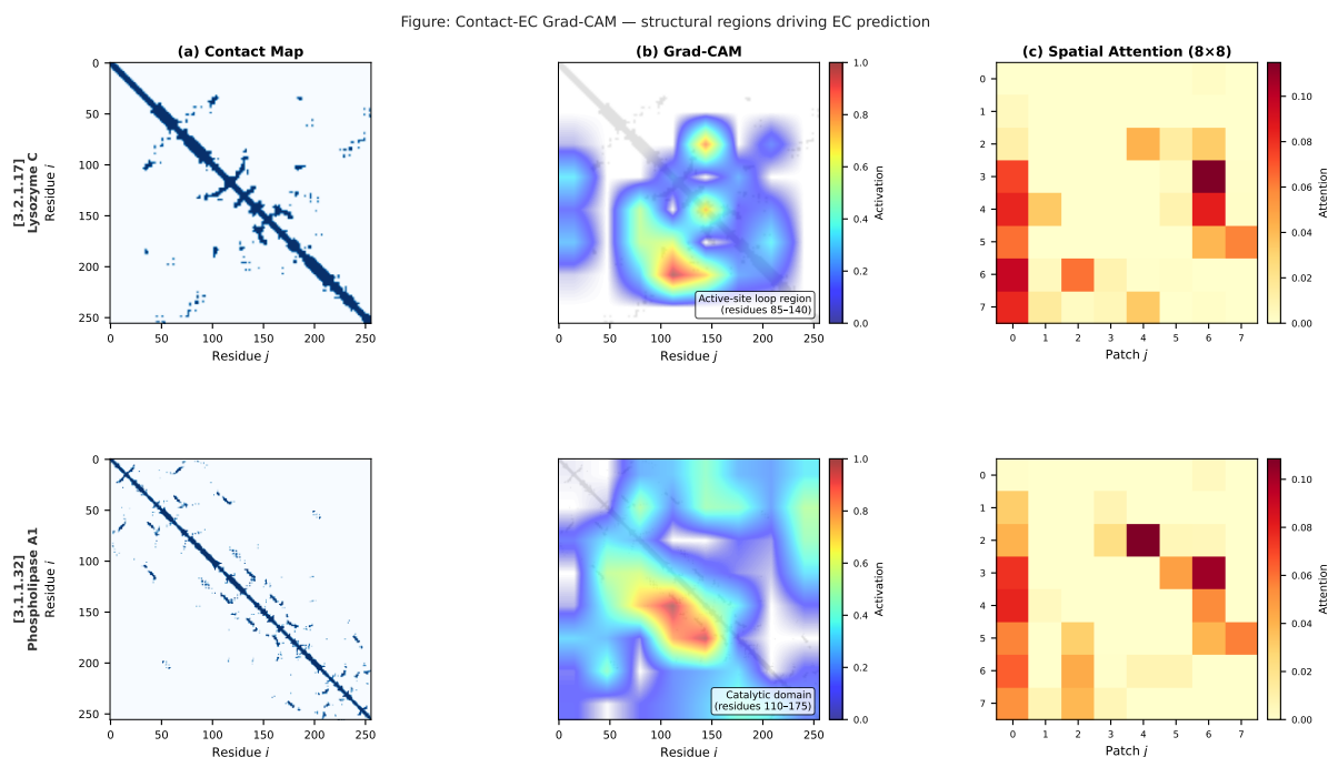
Figure 4: Grad-CAM structural interpretability for Contact-EC. Two correctly predicted test-set enzymes. (a) AlphaFold-derived contact map. (b) Grad-CAM heatmap overlaid on the contact map. (c) ResNet-50 spatial attention weights at the 8 \times 8 feature-map level. Top : Lysozyme C (EC 3.2.1.17, UniProt C0HLB7). Bottom : Phospholipase A1 (EC 3.1.1.32, UniProt P0DPT0).
