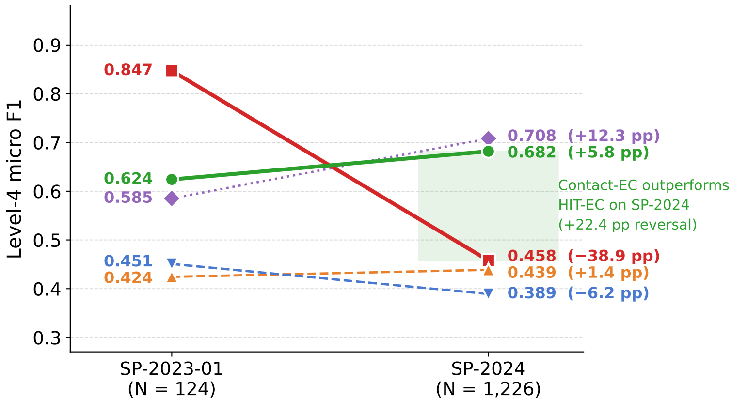
Model trajectories across temporal horizons
