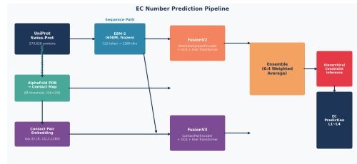
Figure 1 Contact-EC study design for sequence–structure fusion and temporal benchmark decomposition.
