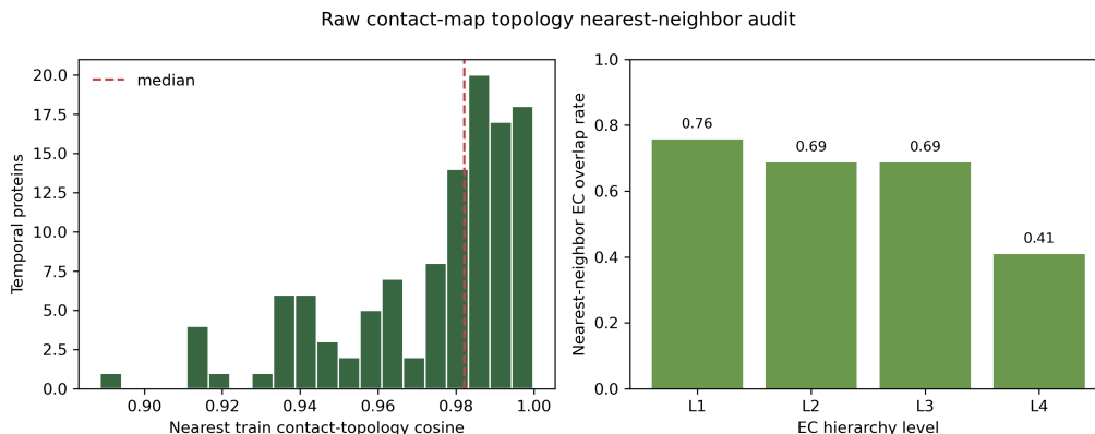
Figure 10: Raw contact-map topology nearest-neighbor audit. Left: nearest SP-2018 training-set cosine similarity for temporal known-EC proteins with available contact maps. Right: EC hierarchy overlap with the nearest topology neighbour.
