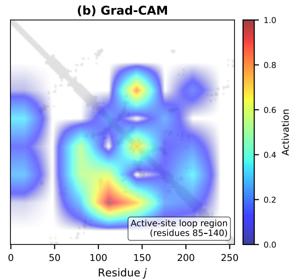
Figure: Contact-EC Grad-CAM — structural regions driving EC prediction
