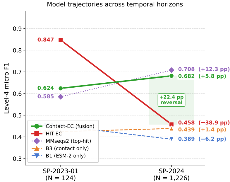
Figure 3 Model trajectories across the two temporal horizons. Each endpoint value and signed change (pp) is annotated in the model's colour. HIT-EC (red) falls -38.9 pp, whereas Contact-EC (green) improves +5.8 pp, producing a +22.4 pp reversal on SP-2024 (shaded region). Thick solid lines: our model and HIT-EC; thin dashed lines: single-modality baselines.
