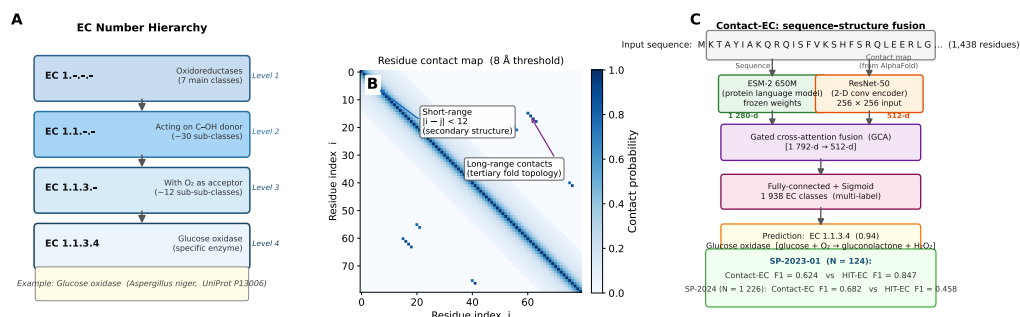
Figure 1 Contact-EC overview. (A) EC number four-level hierarchy illustrated with glucose oxidase (EC 1.1.3.4). (B) Example protein contact map (8 Å threshold); short-range backbone contacts form the diagonal band; long-range contacts (blue arrows) encode tertiary fold topology. (C) Contact-EC pipeline: ESM-2 (1280-d) and ResNet-50 contact-map encoder (512-d) are fused via gated cross-attention before a flat FC sigmoid head predicts all 1,938 Level-4 EC classes simultaneously.
