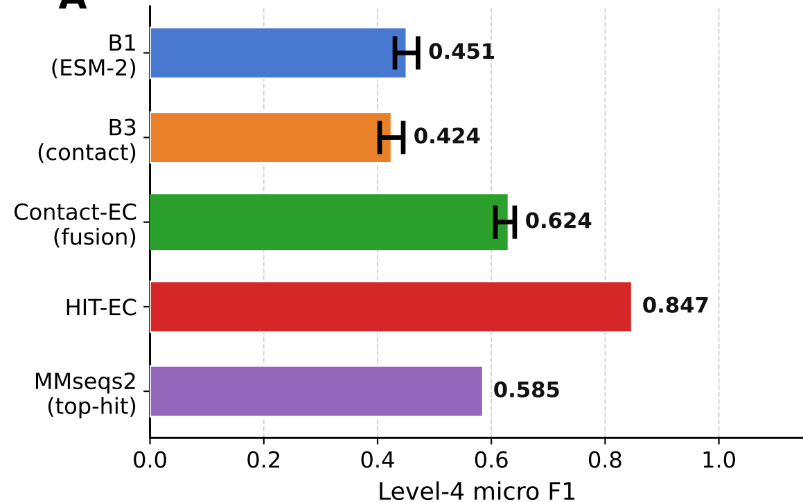
A SP-2023-01 temporal holdout (N = 124)
